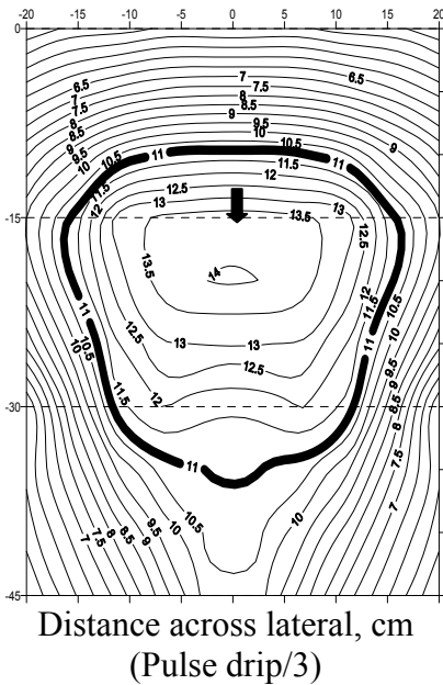
Fig.(5) Effect of pulse subsurface drip irrigation on wetted soil volume (more than or equal 100% of field capacity) at 100% actual irrigation requirements
