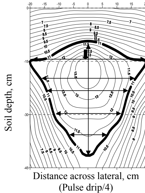
Fig.(5) Effect of pulse subsurface drip irrigation on wetted soil volume (more than or equal 100% of field capacity) at 100% actual irrigation requirements
