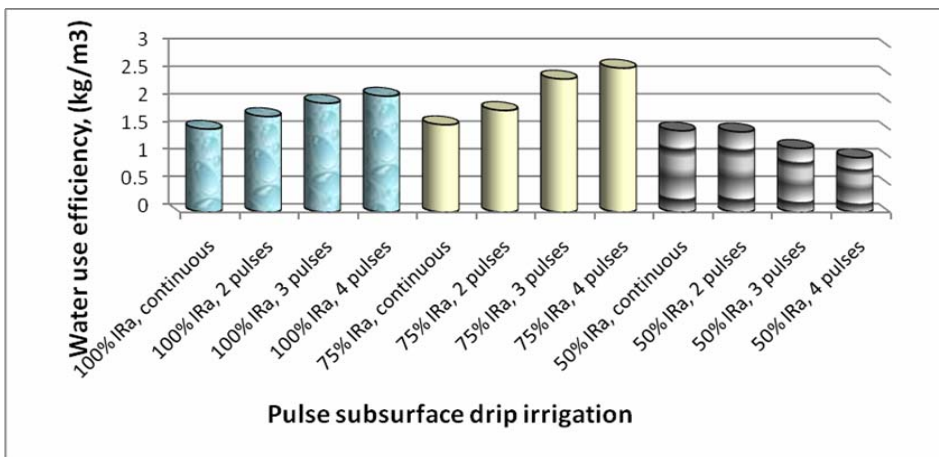
Fig.(15) Effect of pulse subsurface drip irrigation on water use efficiency
