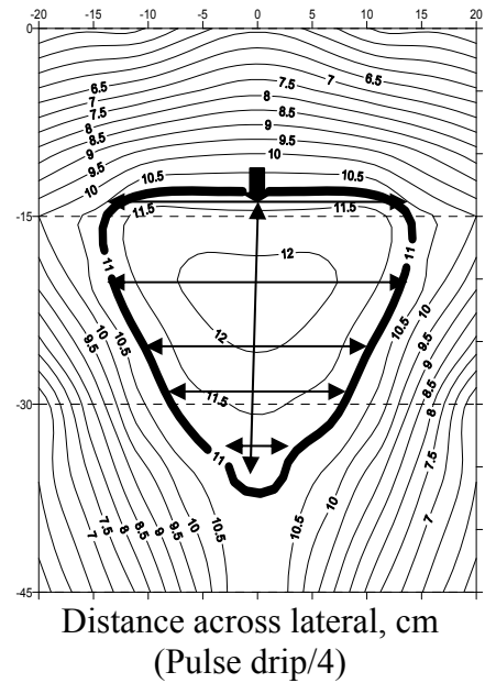
Fig.(7) Effect of pulse subsurface drip irrigation on wetted soil volume (more than or equal 100% of field capacity) at 75% actual irrigation requirements
