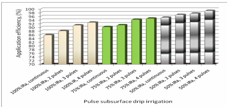
Fig.(11) Effect of pulse subsurface drip irrigation on application efficiency
