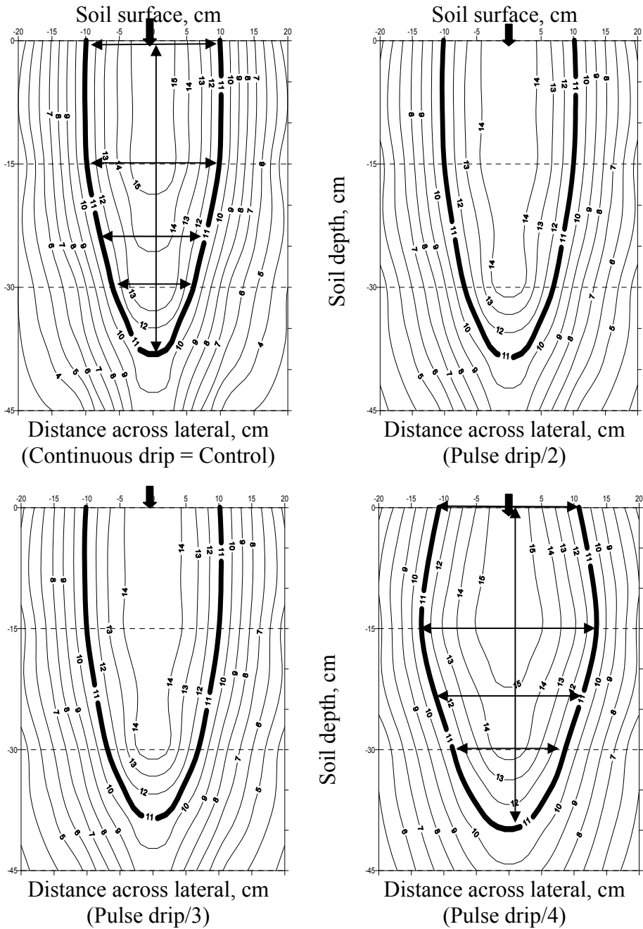
Fig.(6) Effect of pulse surface drip irrigation on wetted soil volume (more than or equal 100% of field capacity) at 75% from actual irrigation requirements
