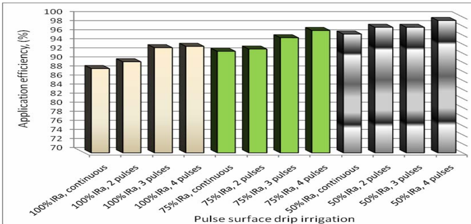
Fig.(10) Effect of pulse surface drip irrigation on application efficiency
