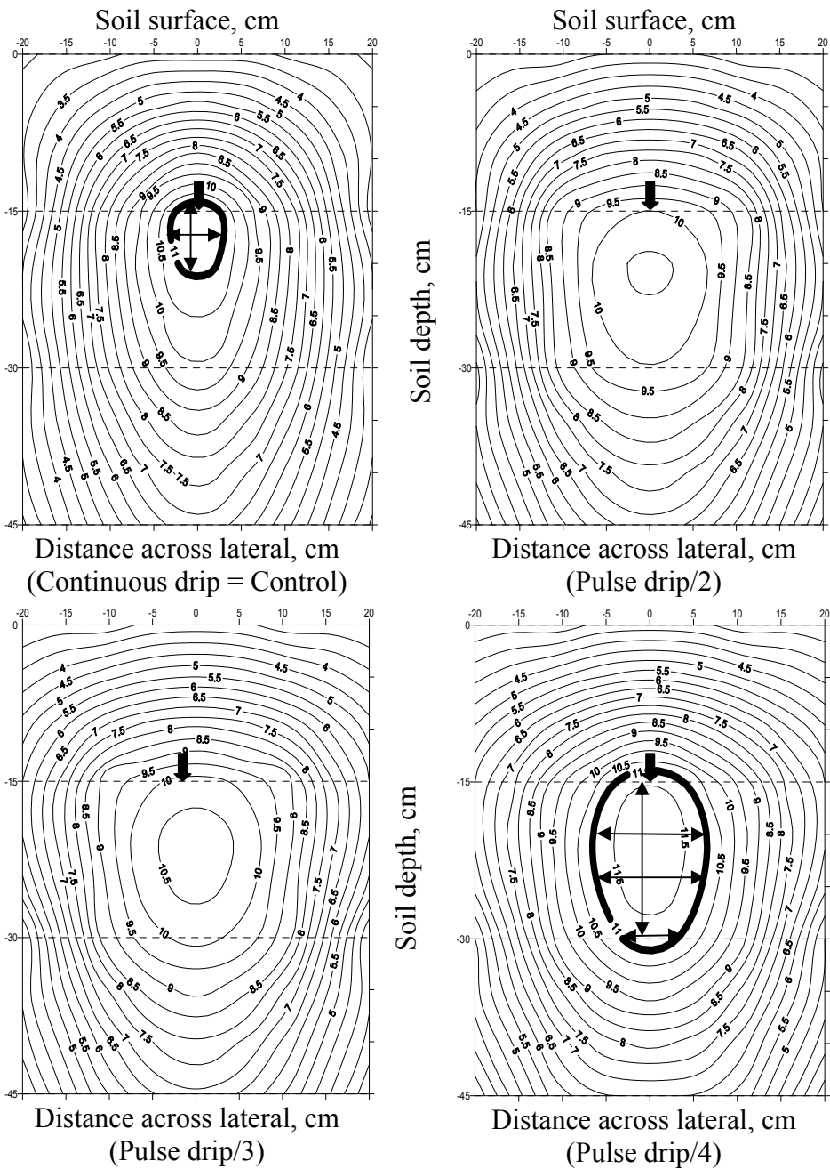
Fig.(9) Effect of pulse subsurface drip irrigation on wetted soil volume (more than or equal 100% of field capacity) at 50% actual irrigation requirements
