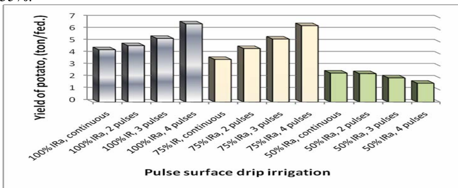
Fig.(12) Effect of pulse surface drip irrigation on yield of potato
