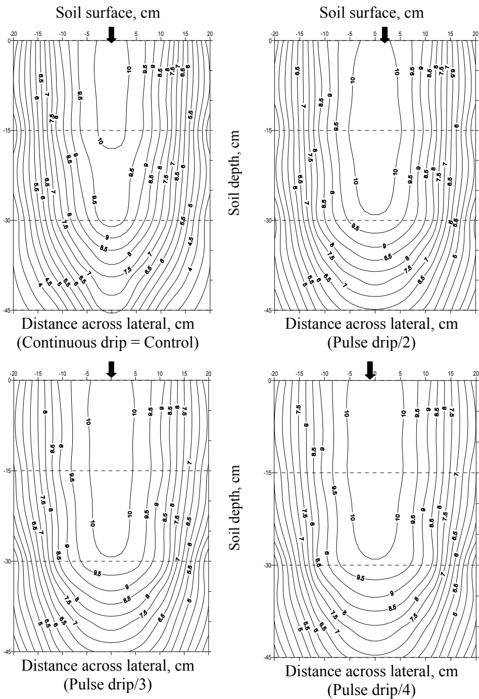
Fig.(8) Effect of pulse surface drip irrigation on wetted soil volume (more than or equal 100% of field capacity) at 50% actual irrigation requirements
