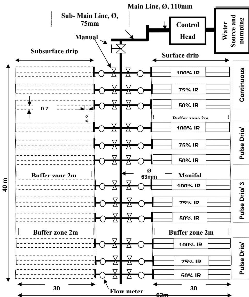
Fig. (2) Layout of irrigation systems with experimental design.
