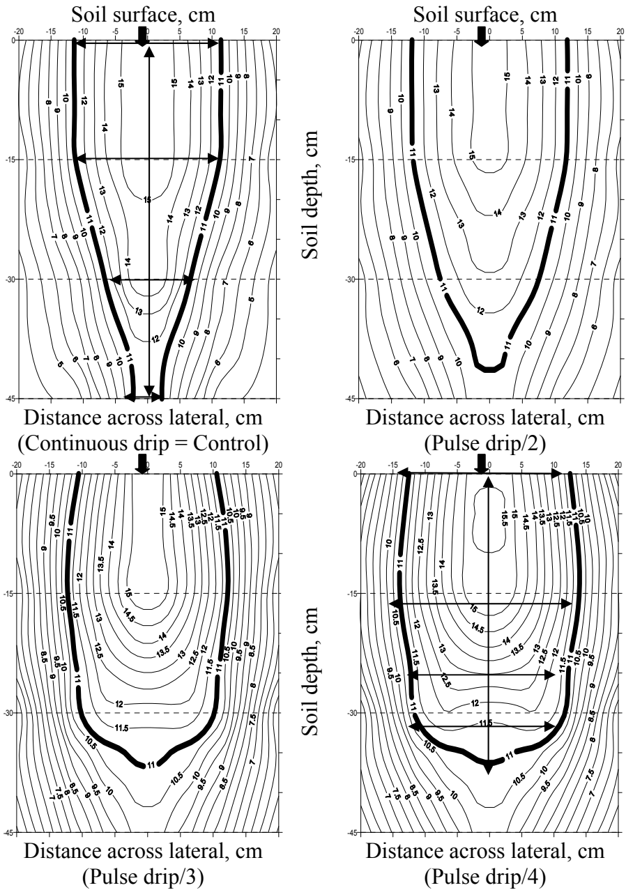
Fig.(4) Effect of pulse surface drip irrigation on wetted soil volume (more than or equal 100% of field capacity) at 100% from actual irrigation requirements
