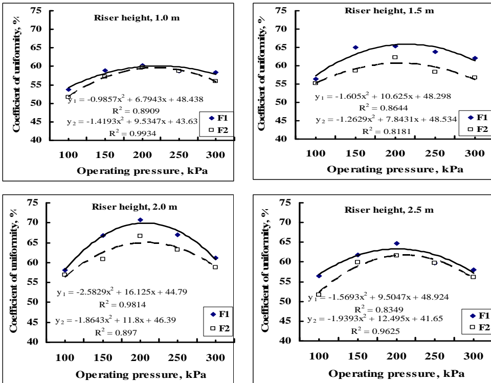
Figure 4: Relationship between operating pressure and coefficient of uniformity at different levels of riser height for the two types of
