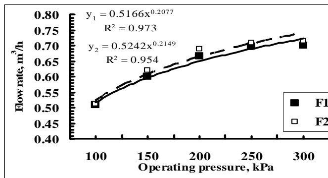
Figure 3: Relationship between operating pressure and flow rate for two types of floppy sprinkler, within the tested domain.
