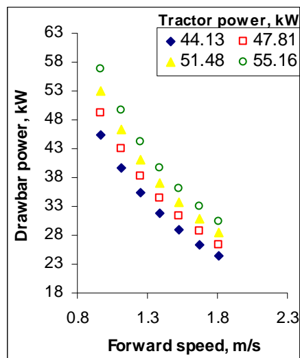
Figure 8: The tractor forward speed via drawbar power.
