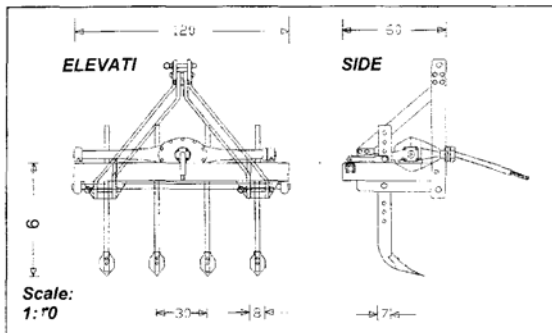
Figure (1): Vibration shanks.
