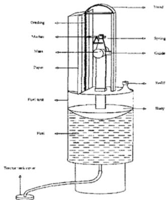
Figure (2): Fuel meter for measuring fuel consumption.
