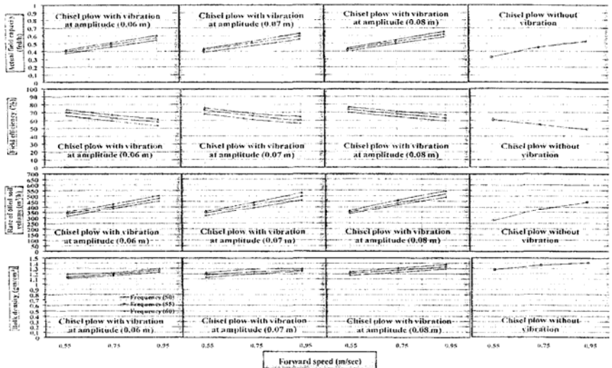
Figure (5): Actual field capacity (fed/h), Field efficiency (%), Rate of tilled volume (m 3 /h) and Bulk density (gm/cm 3 ) at different levels of amplitude, driving force frequency and forward speed in both fixed and vibrated shanks.
