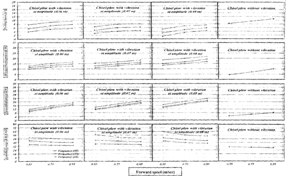
Figure (7): Pulling force (kN), Measurements power (kW), Theoretical power (kW) and Specific energy (kW.h/fed) at different levels of amplitude, driving force frequency and forward speed in both fixed and vibrated shanks.
