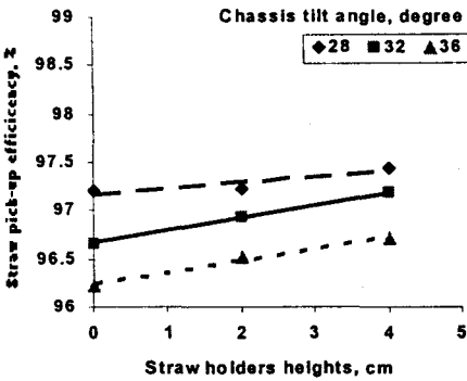
C- Straw holders heights, cm
