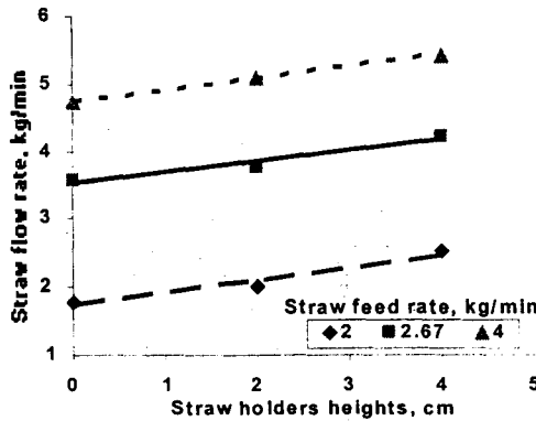
Fig. (5): straw quantity via straw holder height
