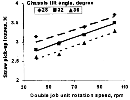
A- Double job unit rotation speed, rpm
