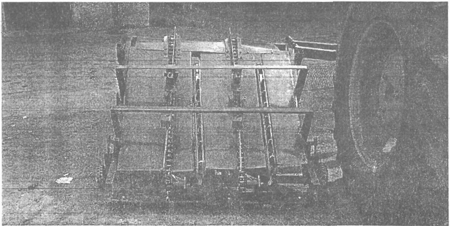
Fig. 2: the side mounted of the machine with tractors
