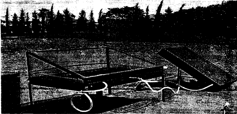
Fig. (1): The solar still system, connected with solar water heater
