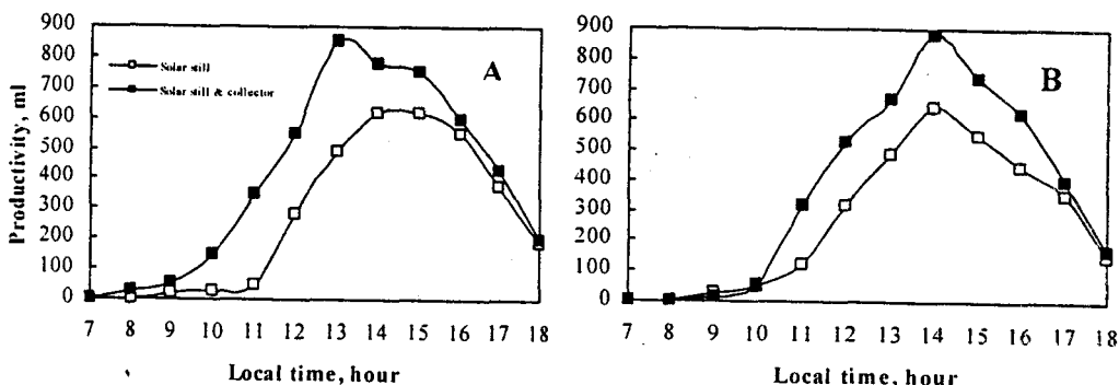
Fig. (7): Comparative variation of still productivity with underground water (A) and saline water (B)
