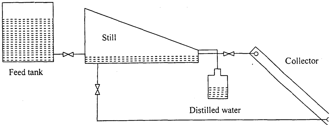
Fig. (2): A schematic diagram showing the arrangement of the still-collector system.
