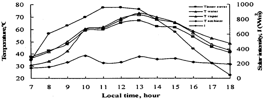
Fig. (5): Hourly variation of temperature for the still alone under saline water feed mode, and the solar radiation.
