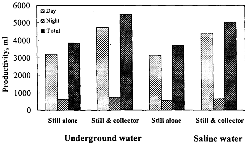
Fig. (8): Comparison of distilled water production at different modes of operation during day and night.
