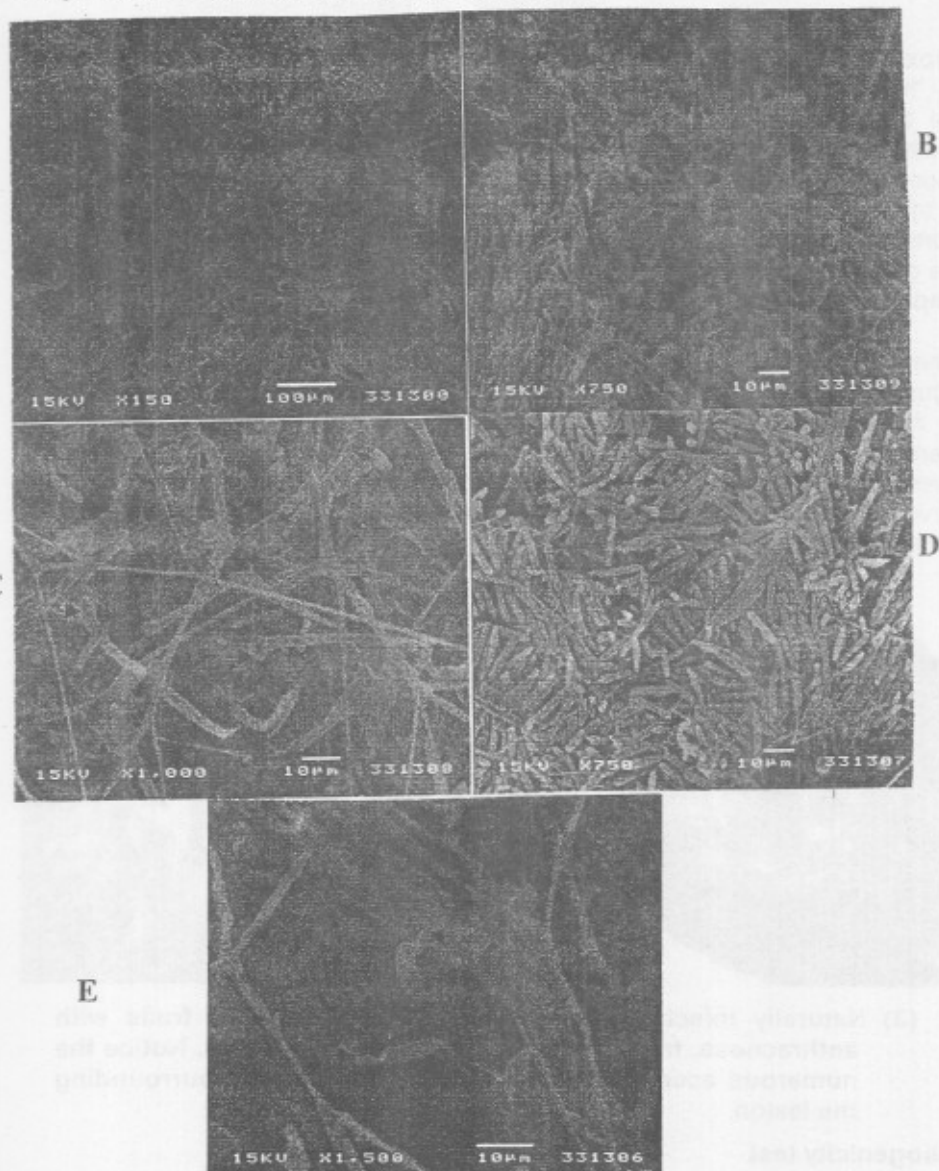
Fig.(2): Scanning electron micrograph showing : acervuli on PDA media 7days old(A), setae and conidia (B),setae slightly swollen at the base and tapered at the apex (C),abundant conidiospores (D) and starting of conidial germinated spores(E)
