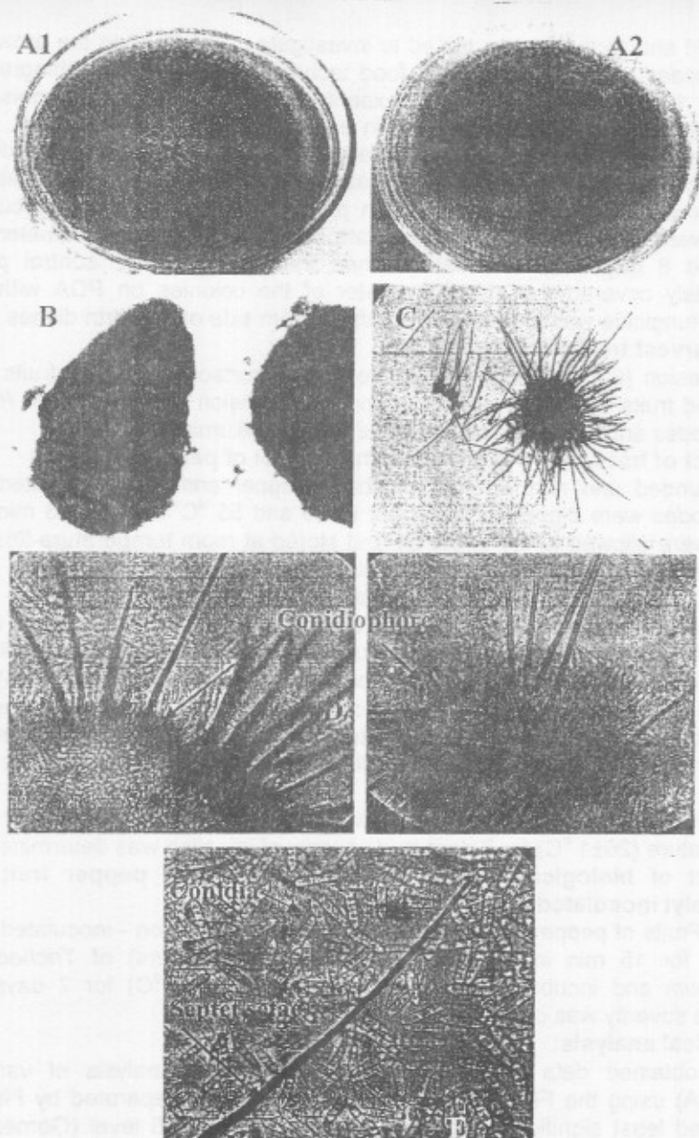
Fig.(1): Morphological characteristics of C.coccodes 10 days old showing the fungal growth on PDA (A 1 ) and on reverses (A 2 ), black microsclerotia (B),acervuli and setae (C),individual acervuli with setae (septate) and conidiophores (D) fusiform shape conidia with acute or pointed ends under light microscope (E).
