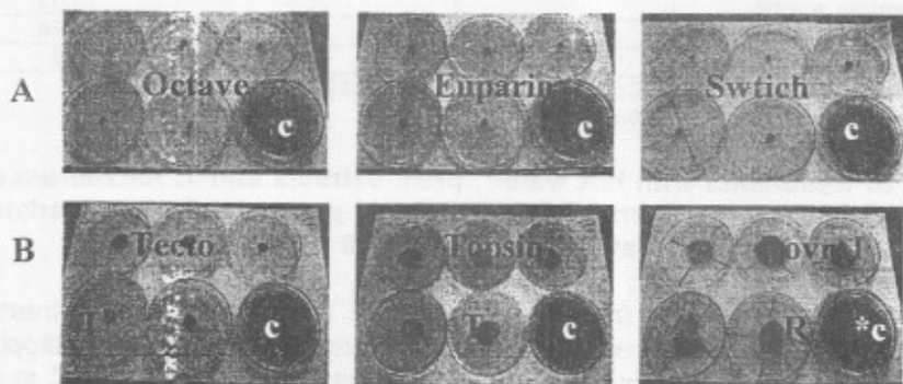
Fig. (5) Showing the effect of different fungicides on the growth of C.coccodes in vitro . Octave, Euparen and Swtich inhibited the growth of the fungus completely at all concentrations tested (A) compared with the Tecto, Topsin and Rovral fungicides (B). *c = control without fungicidal treatment.
