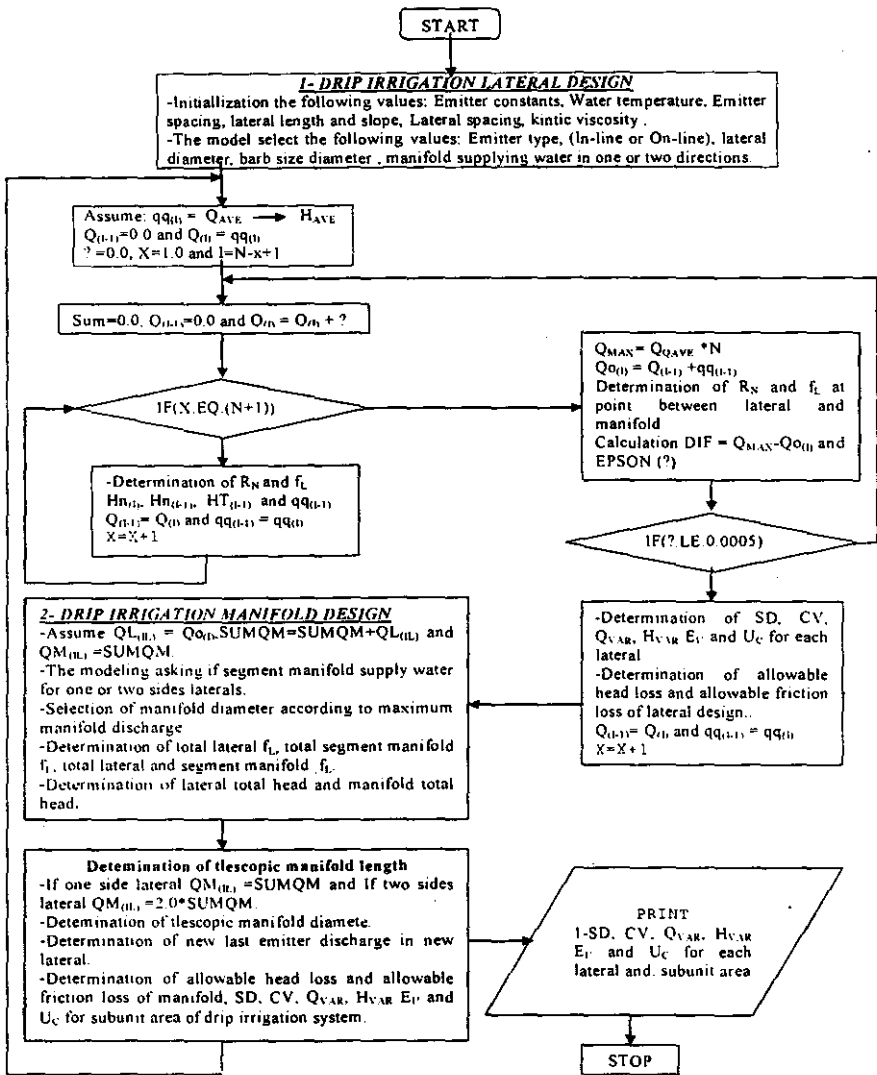
Fig. (1): Subunit drip irrigation design flow-chart
