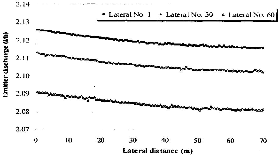
Fig. (2): Measured emitter discharge along lateral distance for lateral No. 1, 30 and 60.
