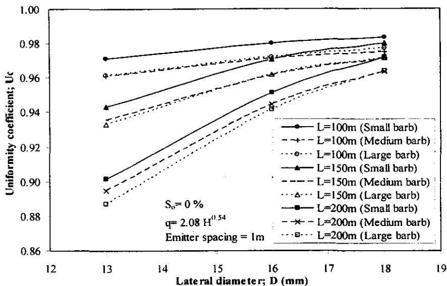
Fig. (8): Uniformity coefficient versus lateral diameter under different emitter barb size diameter and lateral length.
