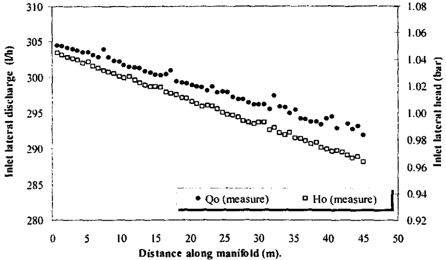
Fig. (3): Measured inlet lateral discharge and inlet lateral pressure head along manifold distance.
