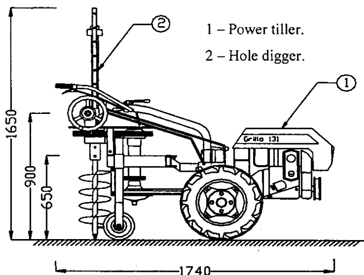
Fig. 1: View of the developed hole digger attached to a power tiller.
