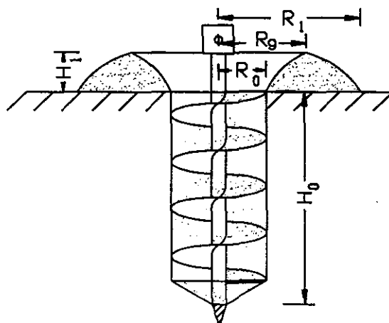
Fig. 3: Hole dimensions.
