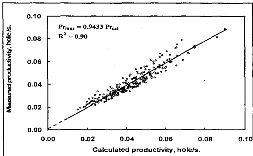
Fig. 6: The relationship between measured ( Pr_{mes} ) and calculated ( Pr_{cal} ) hole-digging productivities.
