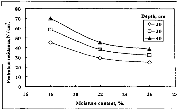
Fig. 4: Penetration resistance for clay soil at different moisture-contents and soil-depths.
