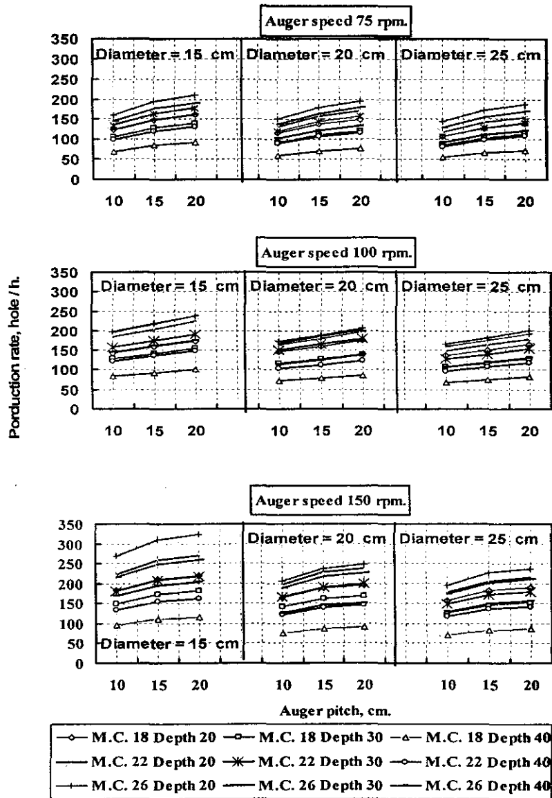
Fig. 5: Effect of auger speed, auger diameter, auger pitch, moisture content (%) and hole depth on hole-digging production rate for clay soil.
