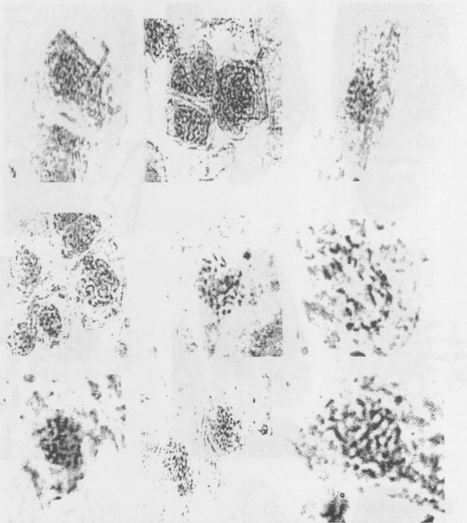
Figure (4): Tetraploid sugar beet young leaf cells at different stages of mitotic division.
