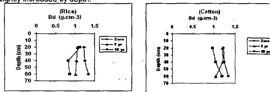
Fig.(4): Bulk density (Bd) of the studied profiles as affected by rice and cotton cultivation for 5 and 10 years.
