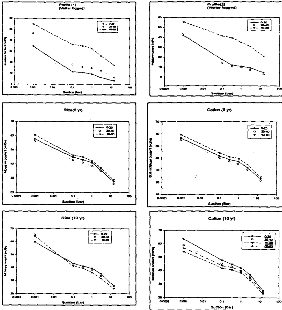
Fig.(7): Moisture characteristics curves of the native wetlands profiles (1 and 2) close to Manzala Lake and those cultivated with rice and cotton.
