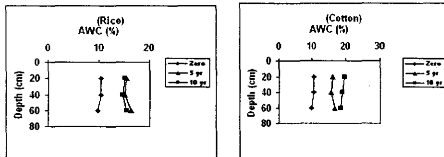
Fig.(8): Available water capacity (AWC) of the studied profiles as affected by rice and cotton cultivation for 5 and 10 years.
