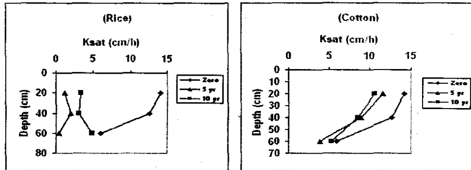
Fig.(5): Hydraulic conductivity ( K_{sat} ) of the studied profiles as affected by rice and cotton cultivation for 5 and 10 years.
