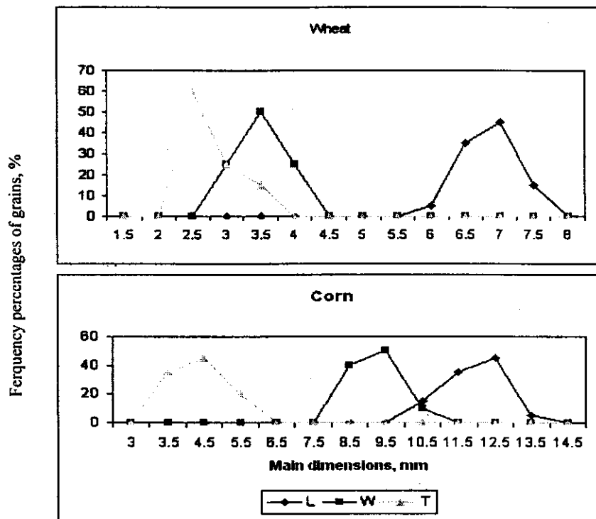
Fig. (1): Frequency of main dimension for different type of grain crops.
