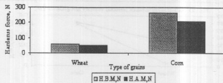
Fig. (7) : Reduction of grain milling force after tempering process.
