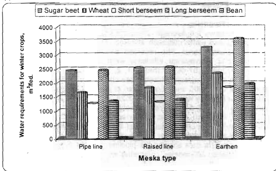
Fig.10: Effect of meska type on water requirements for winter crops during 2005/2006.
