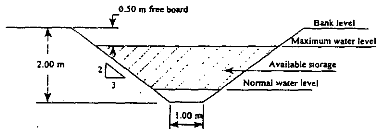
Fig. 4: Layout of an earthen meskas.
