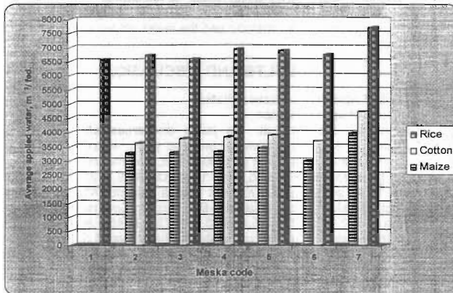
Fig. 6: Effect of Meska type on average applied water for summer crops.
