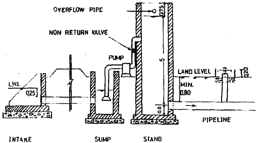
Fig. 2 Sectional elevation of pipe line Meskas layout -Dimension in m- IIP (2003).
