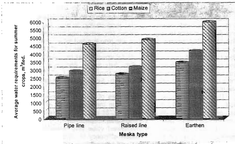
Fig.11: Effect of meska type on water requirements for summer crops during 2006.
