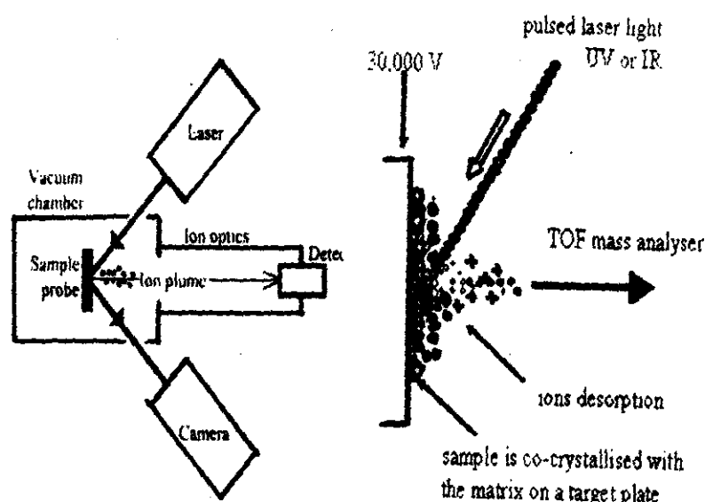
Fig. 1: The ion desorption plume moving from the matrix to the electric field accelerator (Bromhead & Francis 2004)
