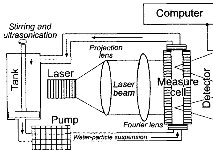
Fig. 4: Main components of a laser diffraction particle size analyzer (Stori & Balsamo 2010)
