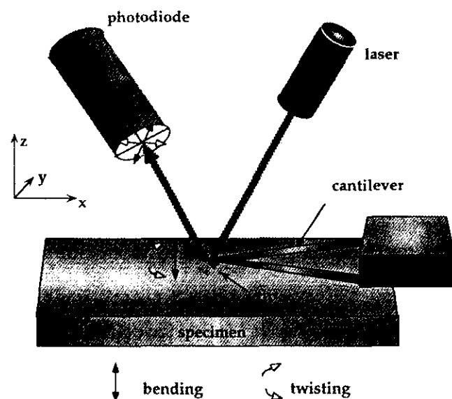
Fig. 3: The basic AFM arrangement presented in schematic form. In this illustration, force detection is via a quadrant detector so that both normal and lateral force measurements can be made (Yang et al. 2007)
