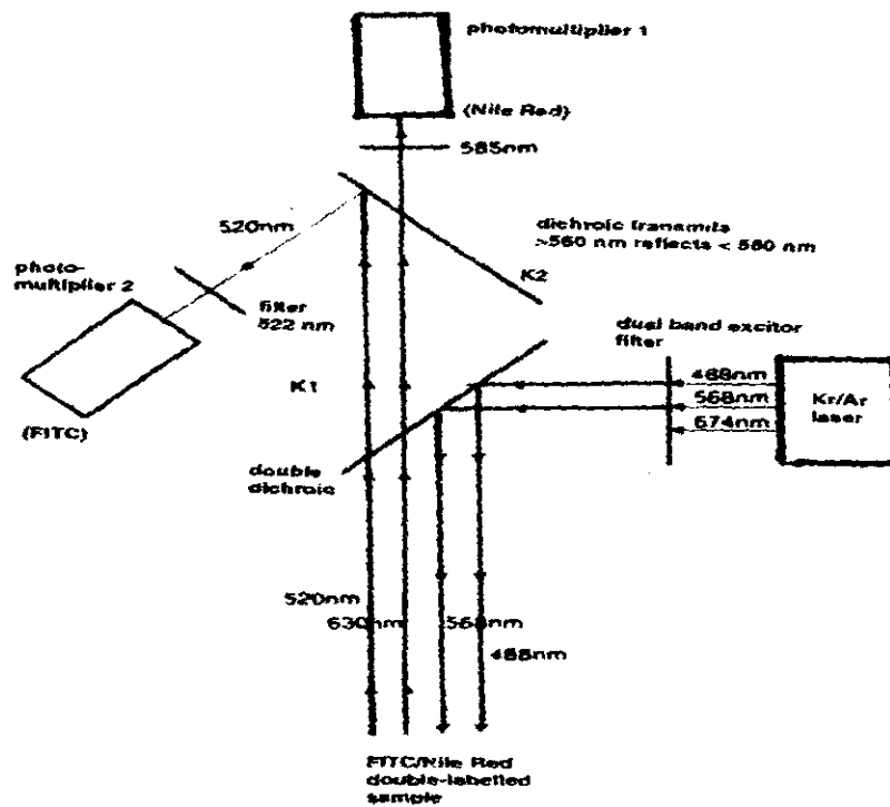
Fig. 2 optical ray diagram for the simultaneous detection of FITC and Nile Red using the orange-krypton mixed-gas laser (adapted from the BioRed MRC600 operating manual) (Renzetti et al. 2008).
