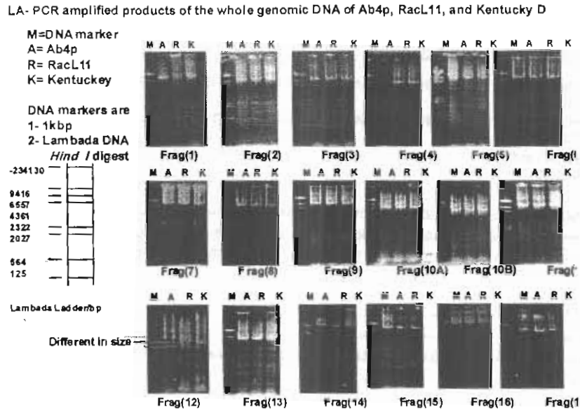
Fig. (2): LA-PCR amplification products of each genome of RacL11, Kentucky D and Ab4P by Agar gel electrophoresis.
