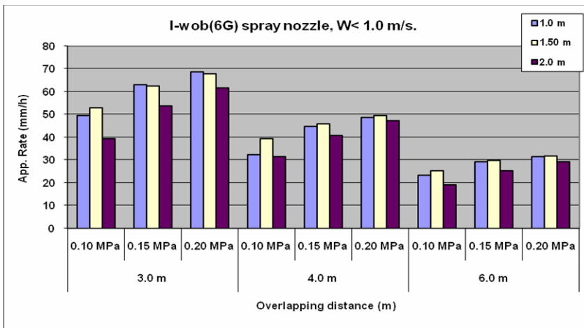
Fig.(11)Average application rate (mm/h) for I-wob (6 G) spray nozzle under different conditions of operating pressures (MPa), nozzle heights (m), overlapping distances (m), at wind speed < 1m/s.
