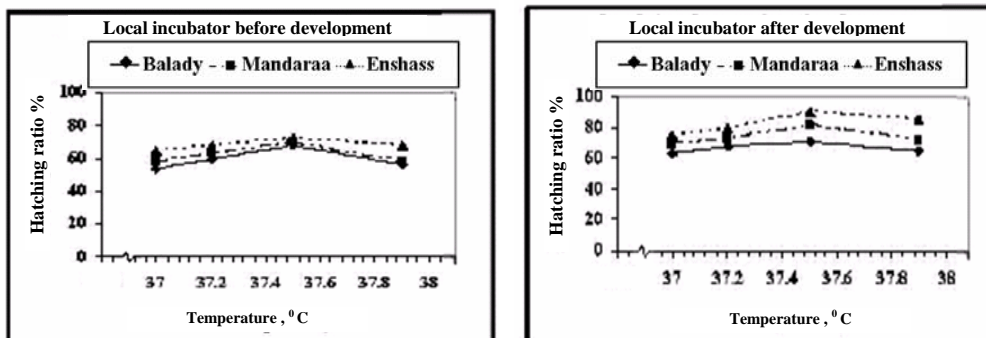
Fig. (6): Relationship between hatching temperature and hatching ratio for local semi-mechanical incubators before and after development using different kinds of eggs.
