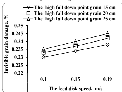
Fig. (4-a) Effect of feed disk speed and high fall down point grain on invisible grain damage.
