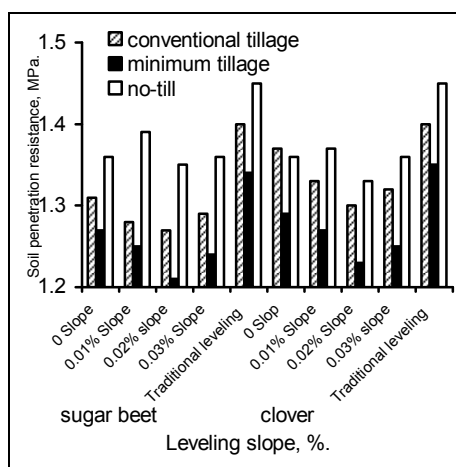
d. Penetration resistance.
