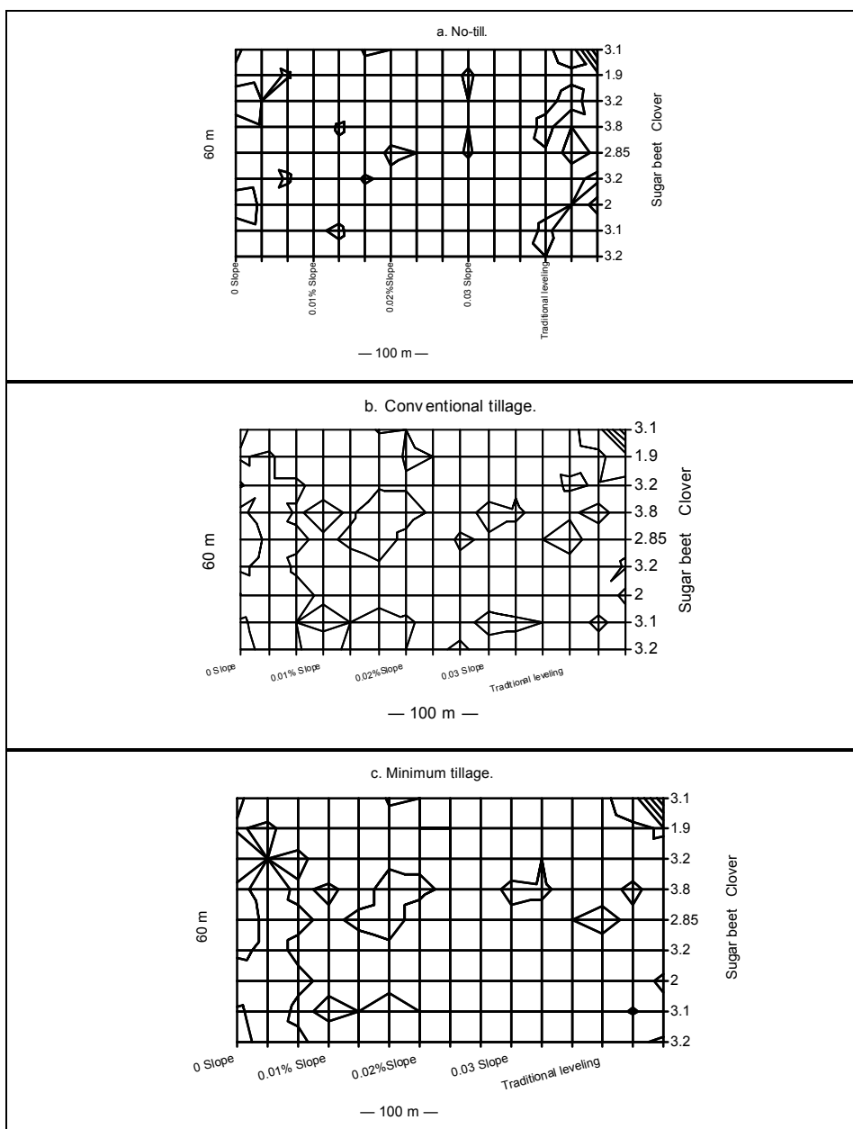
Fig. (4): Schematic diagram of the experimental field grid survey after sugar beet and clover harvest.
