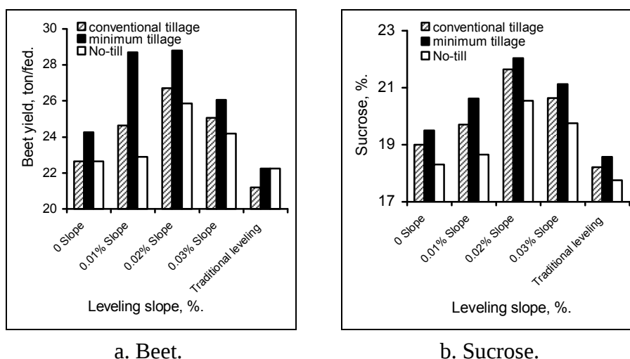
Fig. (5): Effect of minimum tillage on beet and sucrose yield.
