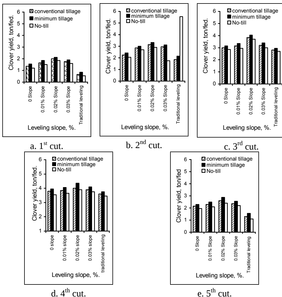
Fig. (6): Effect of minimum tillage on dry clover yield.
