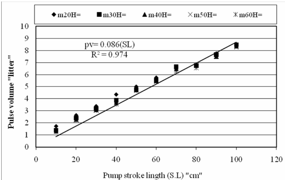
Fig. (9) Relationship between pump stroke length (S.L) "cm" and pulse volume "litter"
