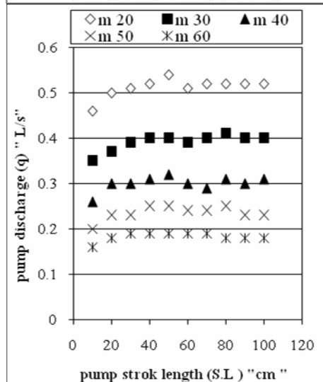
Fig (6) Relation between pump discharge "q" and strok length (S.L) at different pump lift (H).(singl acting)
