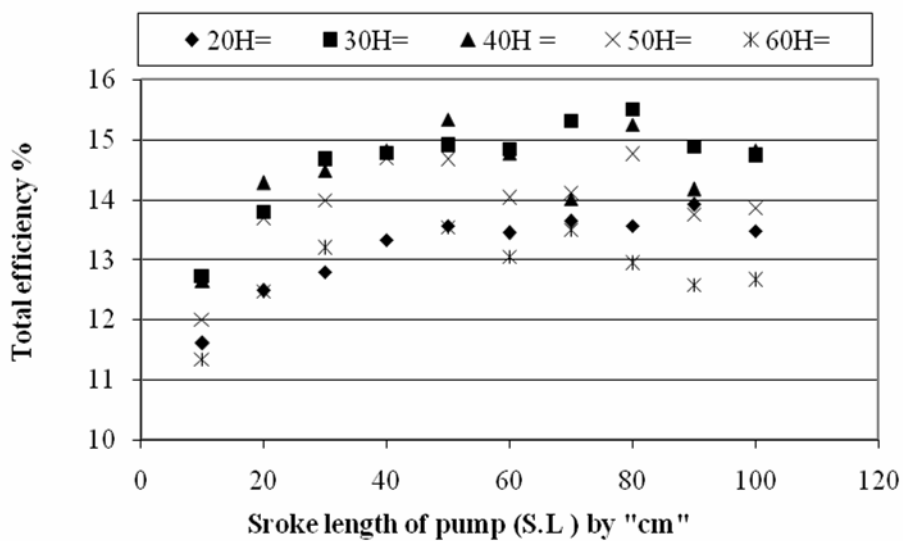
Fig. (8): Relation between stroke length of pump (S.L) "m" and efficiency % for single-acting pump.
