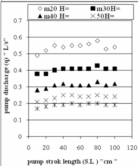
Fig (5) Relation between pump discharge "q" and strok length (S.L) at different pump lift (H).(double acting)
