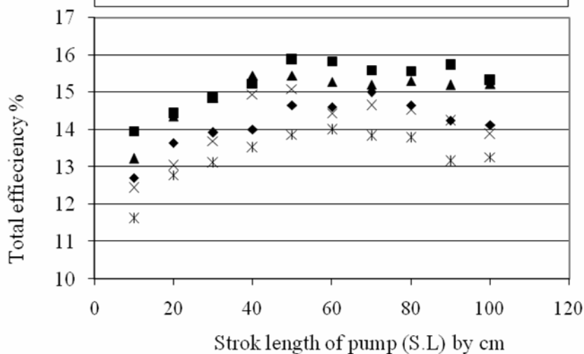
Fig. (7): Relation between stroke length of pump (S.L) "cm" and efficiency % for double-acting pump
