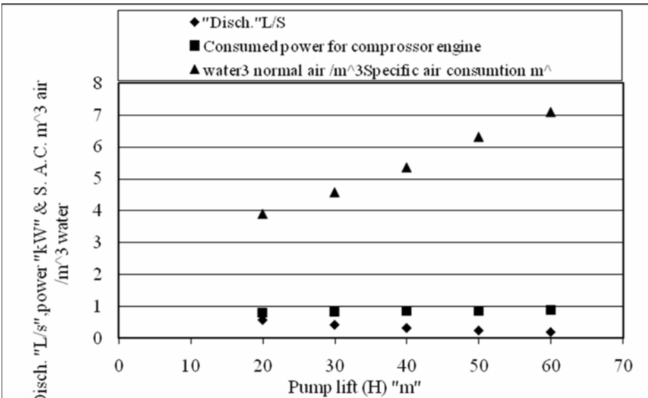
Fig. (10) Relation between pump lift (H) "m" and discharge "L/s", consumed power "kW" and specific air consumption m³ air/m³ water at pump stroke length 80 cm.
