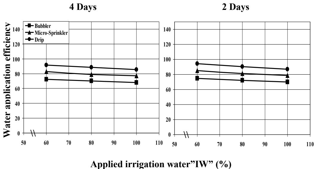
Fig.(4): Water application efficiency "WAE" (%) at applied irrigation water "IW" (%) and different intervals "Int." (Days) for bubbler, micro- sprinkler and trickle irrigation systems on Jatropha .
