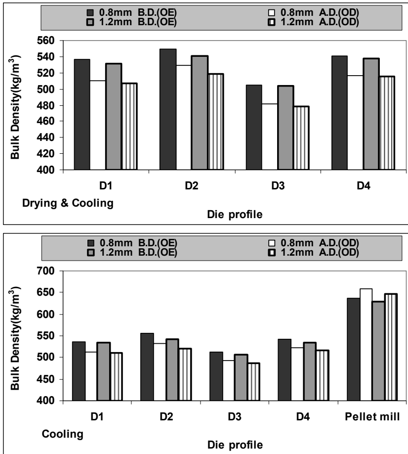
Fig (8A&B) Effect o die pofile, formula particle size after extruded OE and after cooling OD on pellet bulk density.
