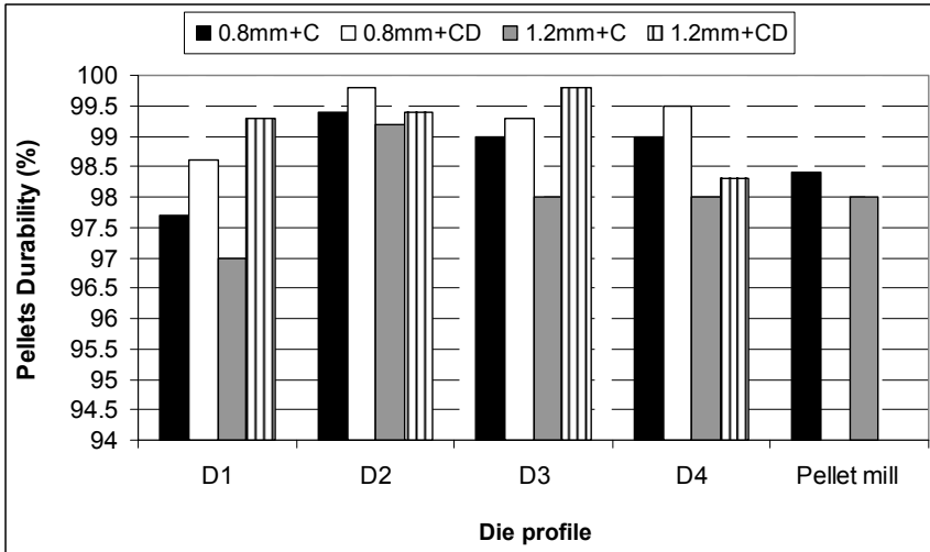
Fig(9) Effect of die holes profile, formula particle size and cooling and drying on pellets durability
