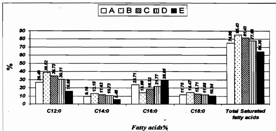
Fig. (1): Saturated fatty acids composition of five Egyptian biscuit fat.
