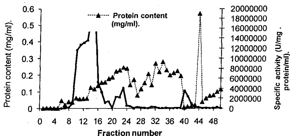
Fig. 2. Fractionation pattern of protease(s) produced by B. licheniformis B-42 at 55°C using sephadex G-200 column chromatography technique.
