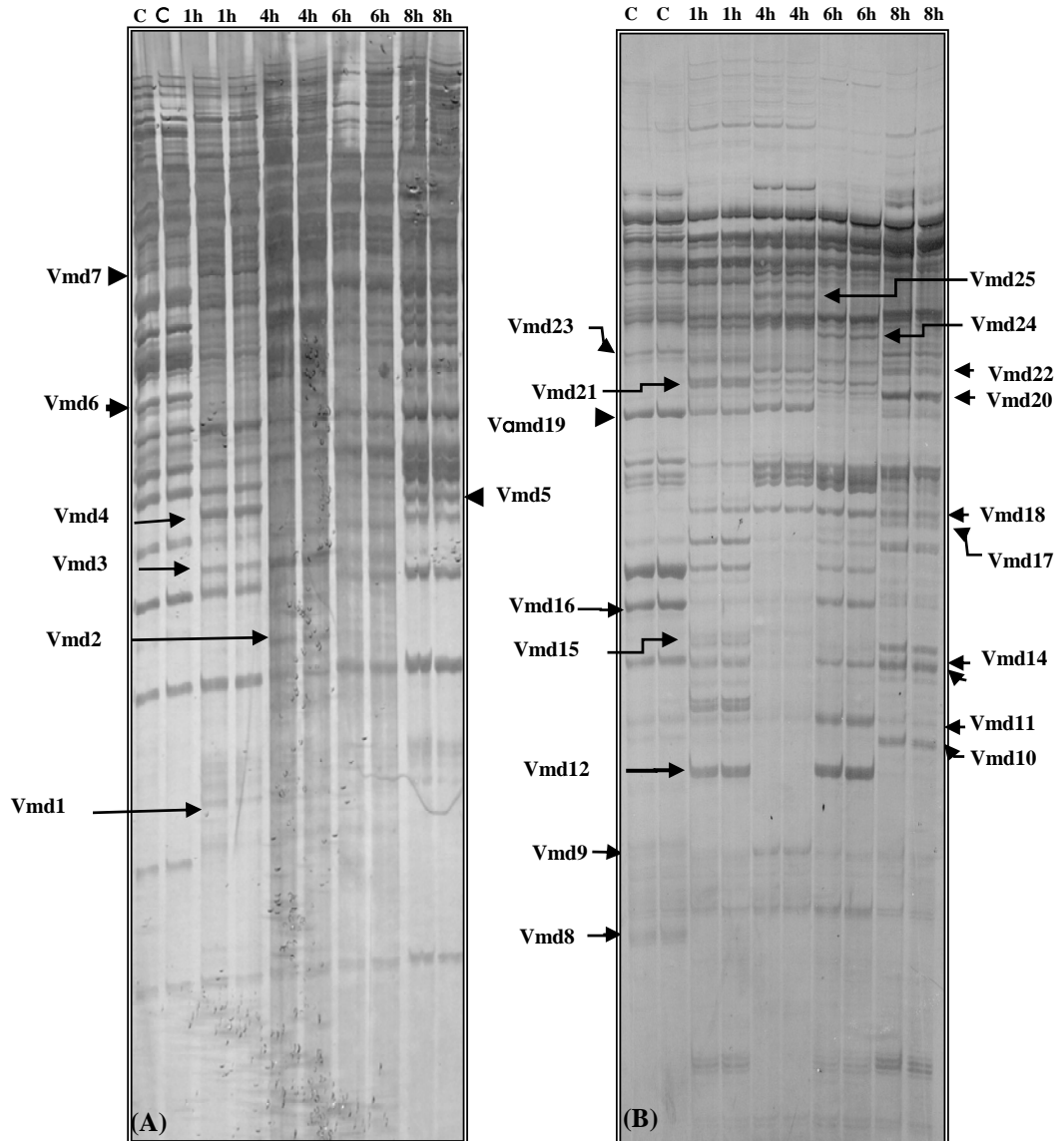
Fig. (1): DD-polyacrylamide gels of shoot cDNAs under control(c) and stress (1, 4, 6 and 8 h) conditions utilizing different primer combinations, A) T11A with AP5 and B) T11G with AP5. Arrows indicate a number of differentially expressed bands on a duplicate basis.
