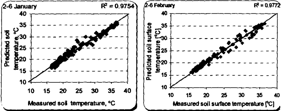
Fig.15: Comparison measured and predicted of the soil temperature 3.5 The Relative Humidity.
