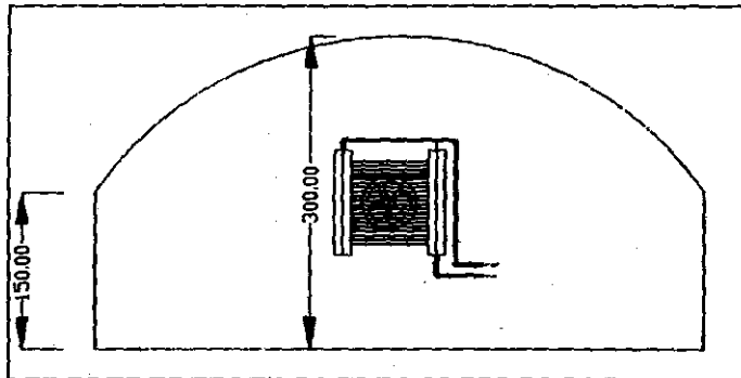
Fig.3-b: Elevation of the greenhouse used in the experimental study.
