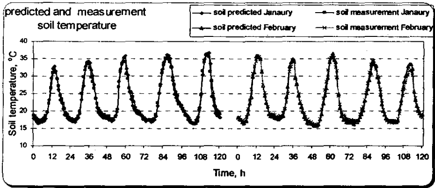
Fig.13: predicted and measured soil temperature.
