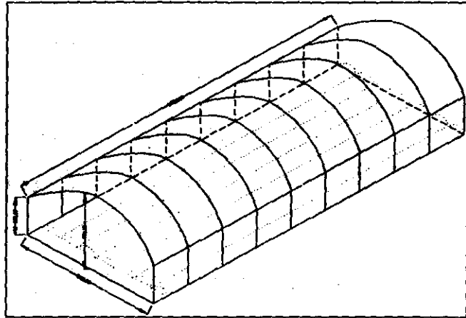
Fig.3-a: Isometric view of the greenhouse used.
