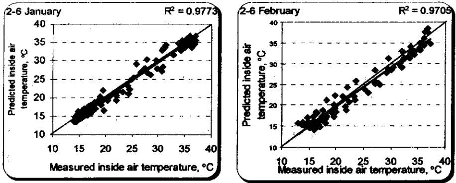
Fig.6: Comparison between measured and predicted of the inside air temperature.
