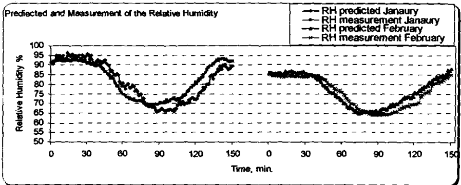
Fig.16: predicted and measured relative humidity.
