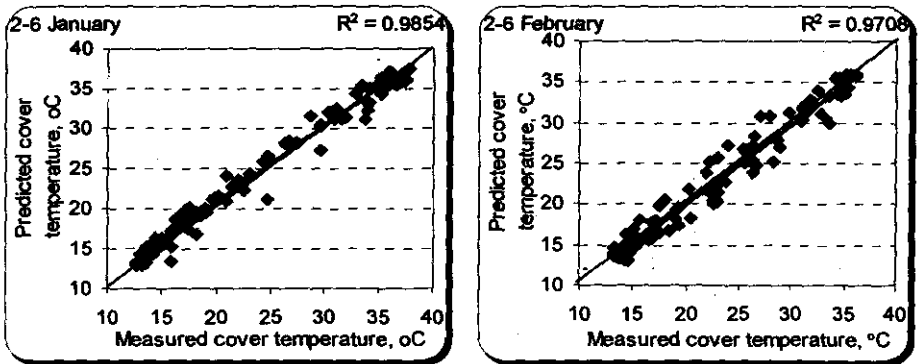
Fig.12: Comparison between measured and predicted of the cover temperature.
