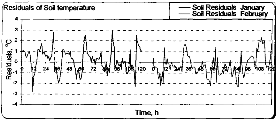
Fig.14: Residuals of the measured and predicted soil temperature.
