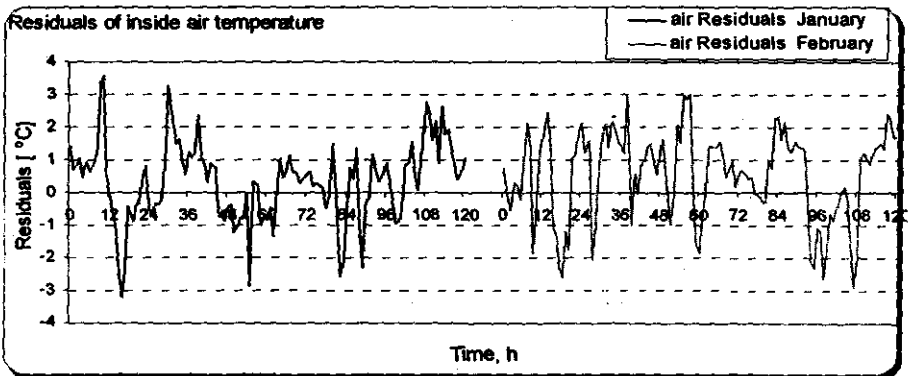
Fig.5: Residuals of the measured and predicted inside air temperature.
