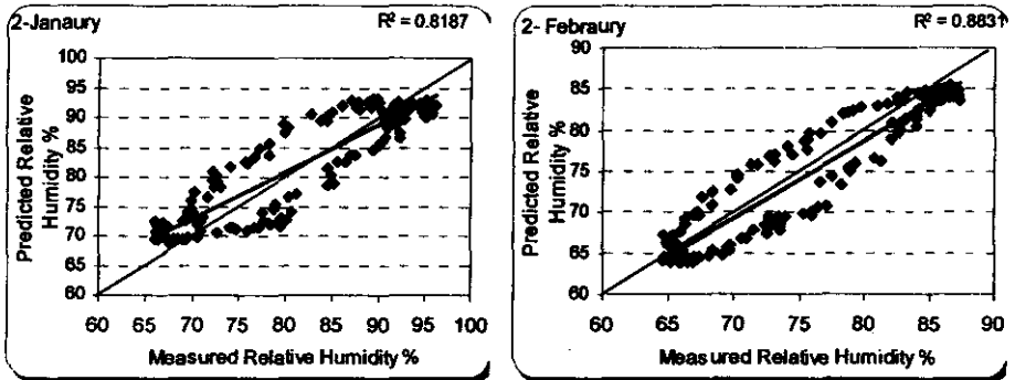
Fig.17: Comparison between measured and predicted of the relative humidity.
