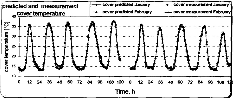
Fig. 10: predicted and measured cover greenhouse temperature.
