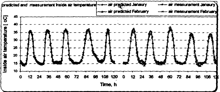
Fig.4: predicted and measured inside air temperature of the greenhouse.
