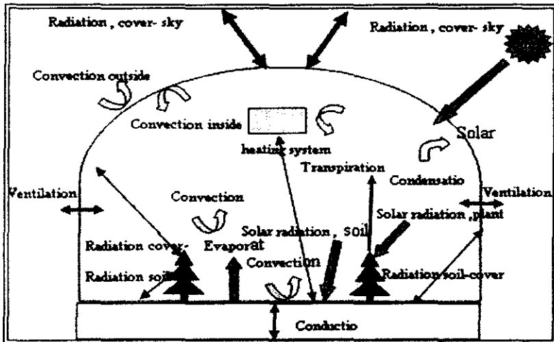
Fig.1: Energy balance and fluxes of the all components of the greenhouse.
