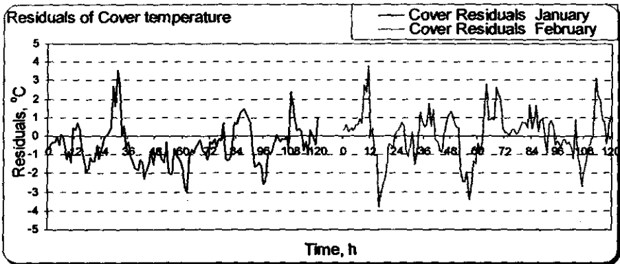
Fig.11: Residuals of the measured and predicted cover temperature.
