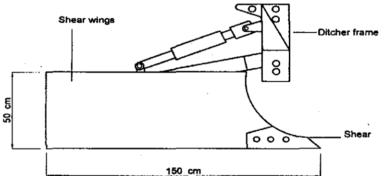
Fig. (1): The outlook of ditcher components.
