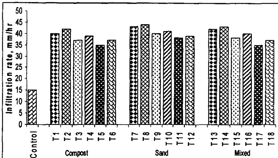
Fig. 3: Infiltration rate values at different treatments.
