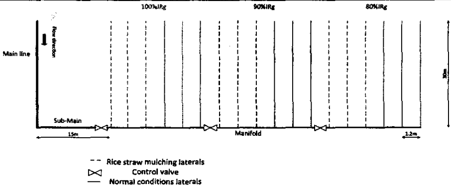
Fig.1: Schematic diagram of the used drip irrigation network
