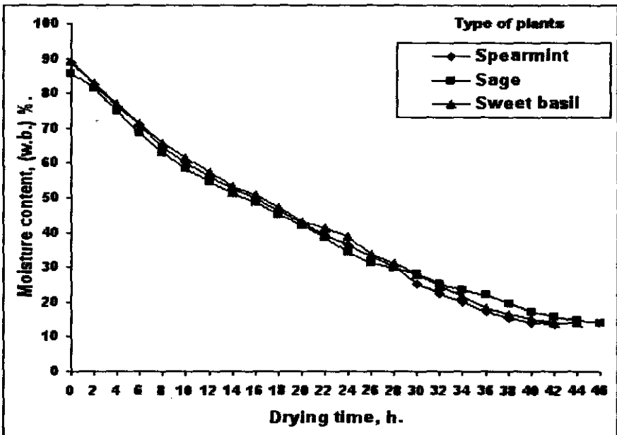
Fig. (2): Change of moisture content as related to drying time for natural drying method
