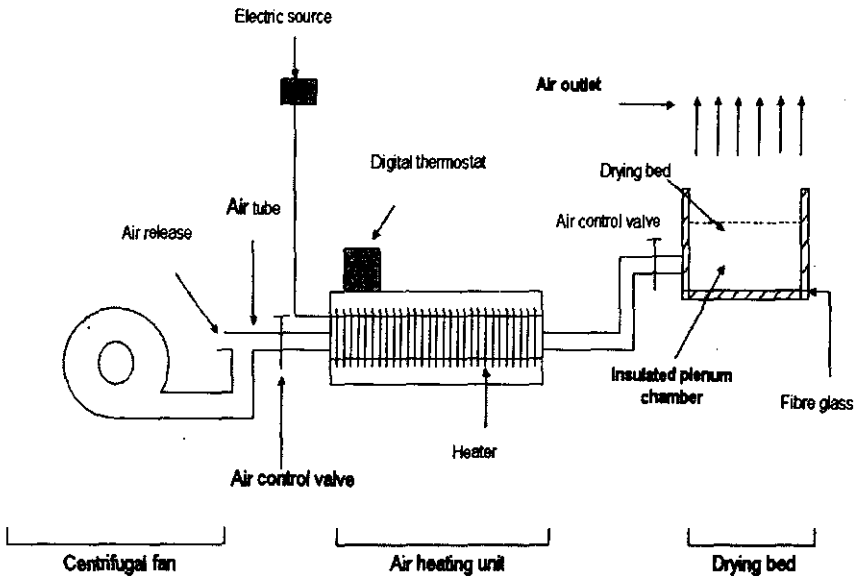
Fig. (1): Schematic diagram of the experimental dryer.
