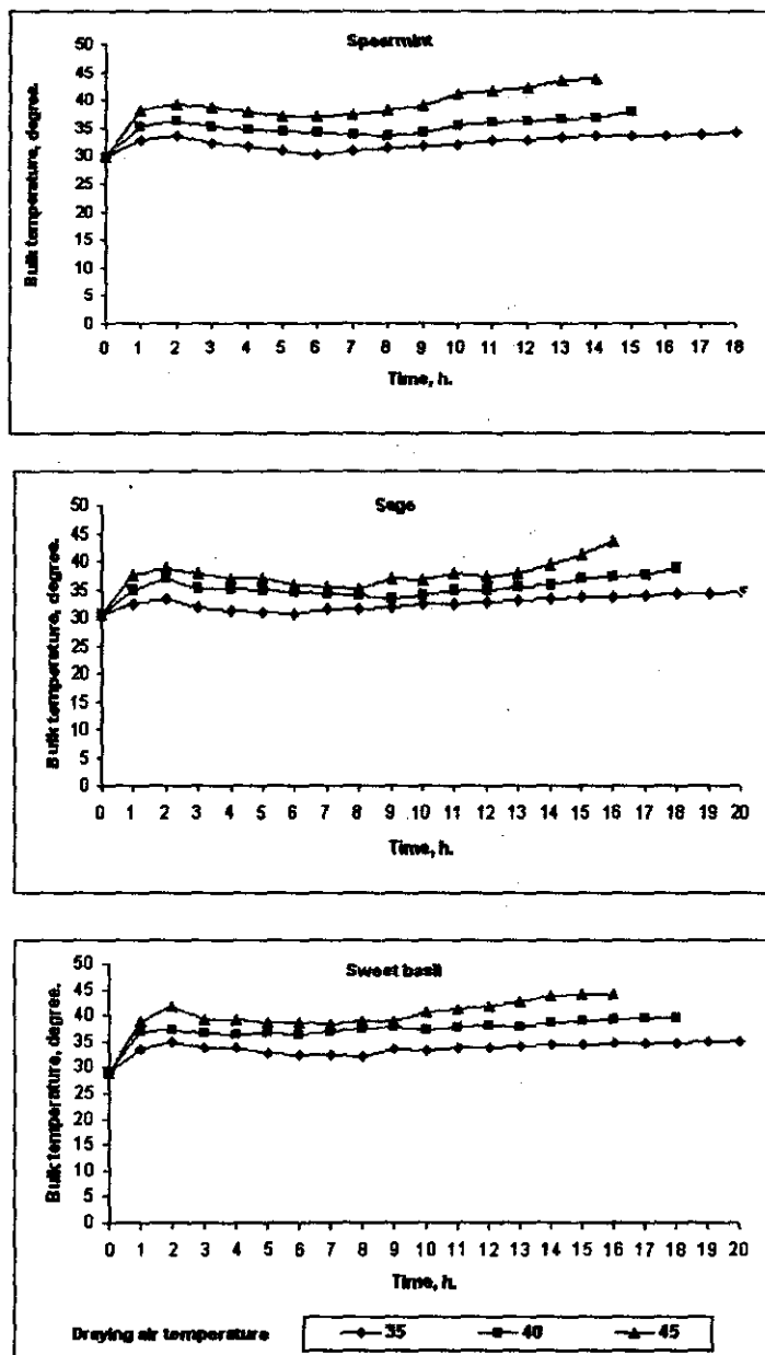
Fig. (3): Change in bulk temperature as a function of drying time for different studied plants.
