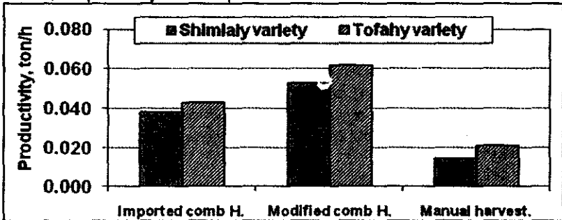
Fig.(6): Labor productivity sustained with olive comb harvester compared with olive manual harvesting method.
