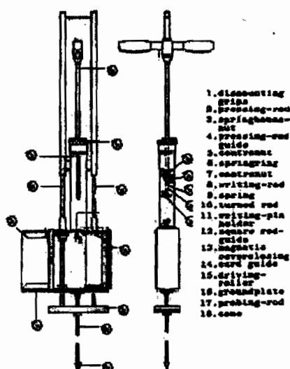
Fig. 1: Penetrograph.
