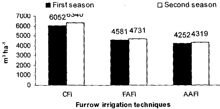
Fig. (1): Effect of different furrow irrigation techniques on the total amounts of irrigation water applied ( \text{m}^3 \text{ha}^{-1} )
