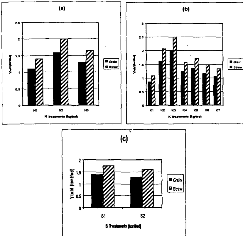
Fig. (1): Effect of N, K and S treatments on grain and straw yield of wheat
