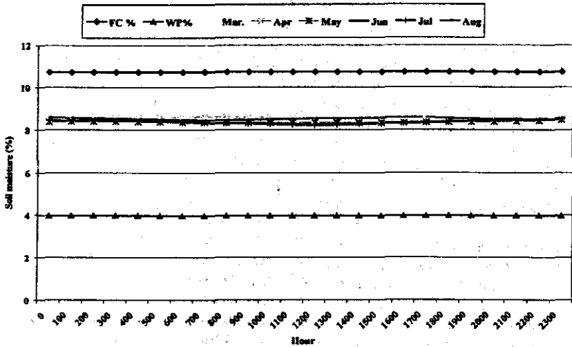
Fig. (2) Daily variations in soil moisture (%) under tomato plants grown in El-Sheikh Zuwaid region.
