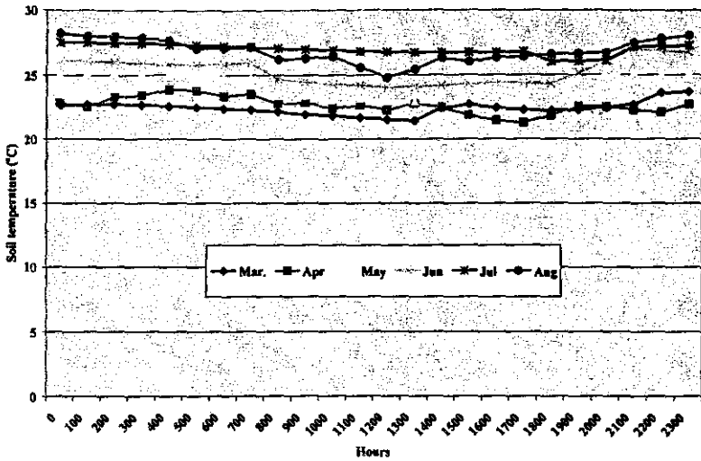
Fig. (3) Daily variations in soil temperature (°C) under olive trees grown in El-Sheikh Zawaid region.
