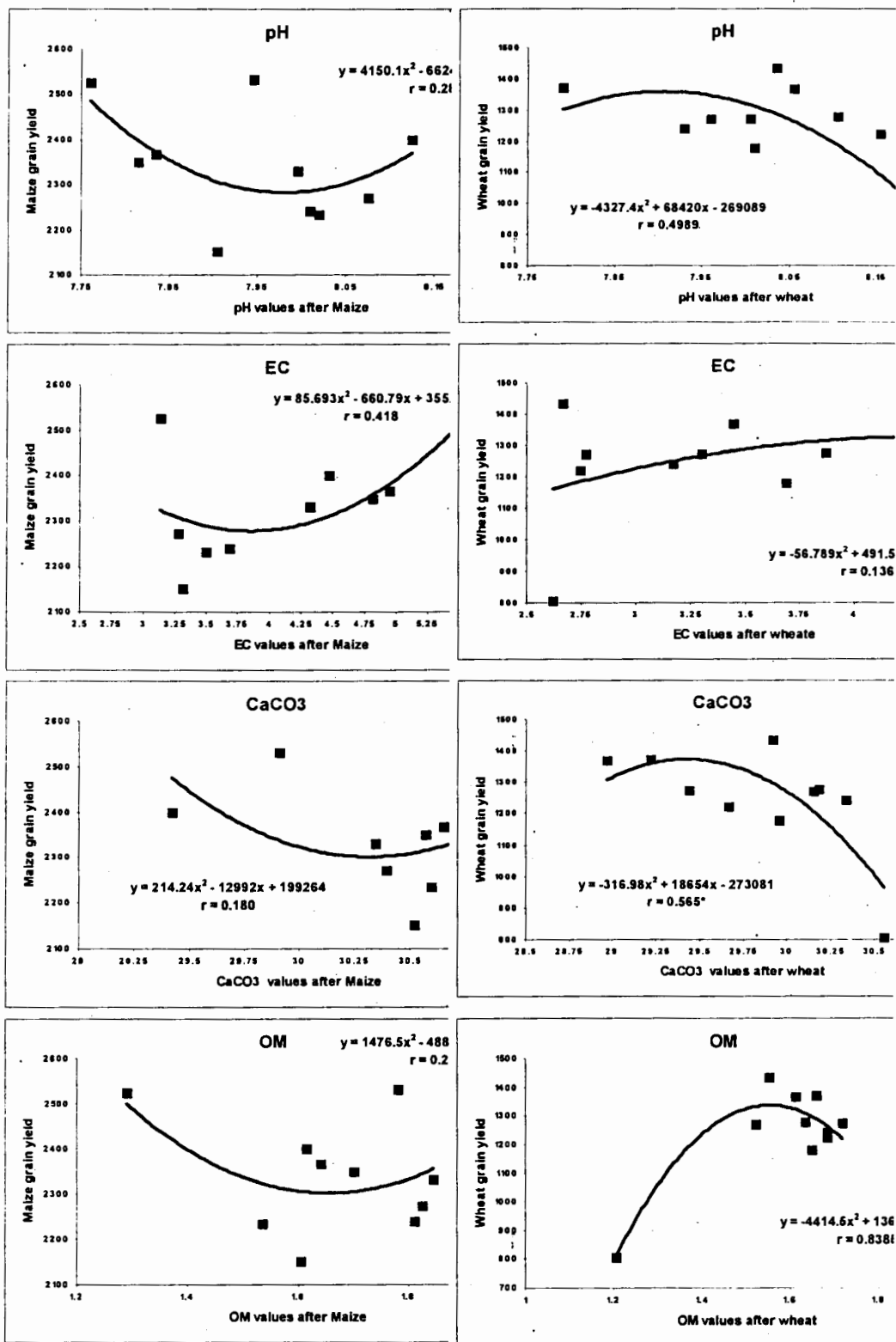
Figure 1. Correlation coefficient values between some chemical properties values for maize and wheat grains together with the corresponding equations.
