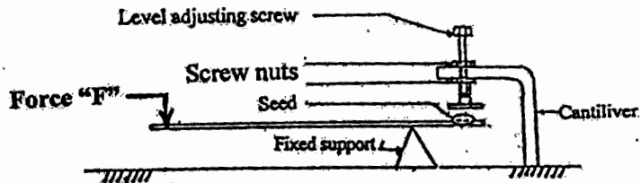
Fig.(1): Apparatus used for fracturing the seed
