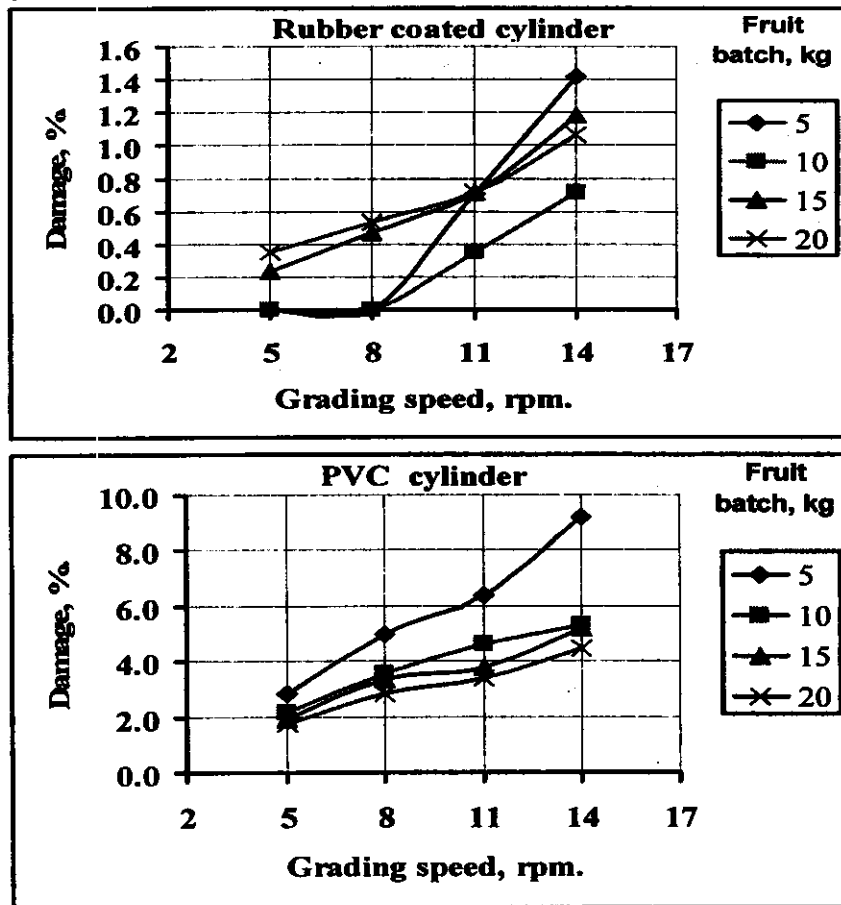
Fig.6: Effect of grading speed, fruit batch and type of grading cylinder (P.V.C. cylinder and rubber coated cylinder method) on fruit damage.
