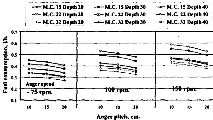
Fig. 8: Effect of auger speed, auger pitch, moisture content (%) and hole depth on fuel consumption of digging the sandy soil.
