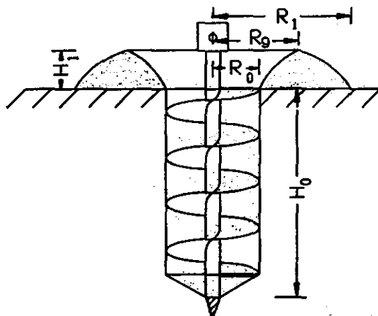
Fig. 4: Hole dimensions.
