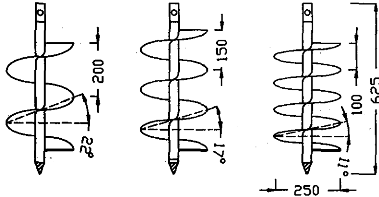
Fig. 2: The Auger of different pitches 100, 150 and 200 mm.
