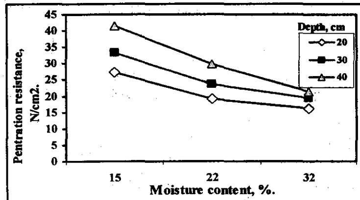
Fig. 5: Penetration resistance for sandy soil at different moisture-contents and soil-depths.
