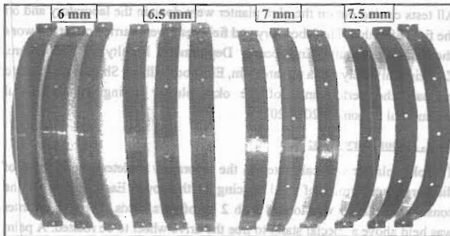
Photo 2. The strips with different metering bores.
