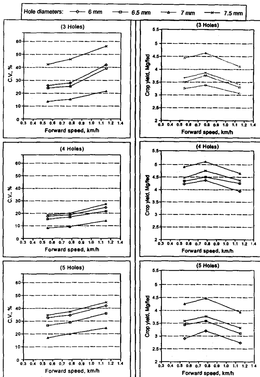
Fig.(6): Effect of machine forward speed on C.V. at different hole diameters and different No. of holes on the hoppers.
