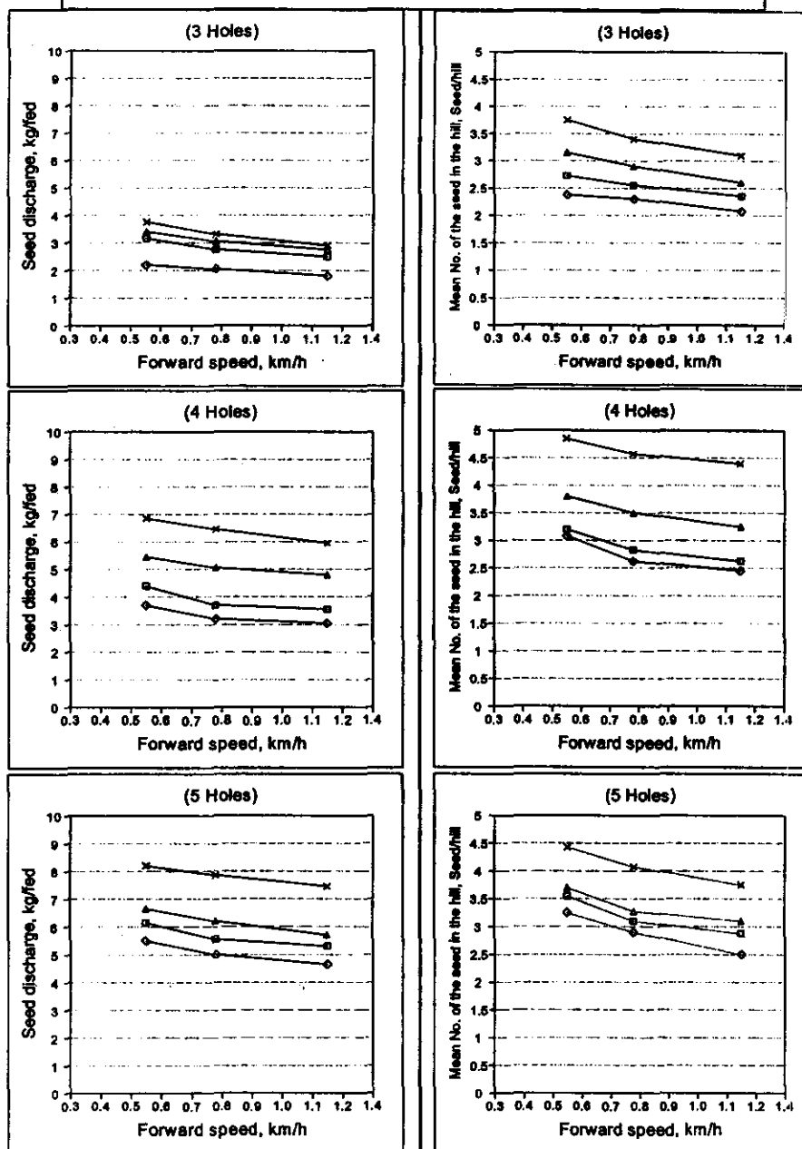
Fig.(4): Effect of machine forward speed on seed discharge at different hole diameters and different No. of holes on the hoppers.
