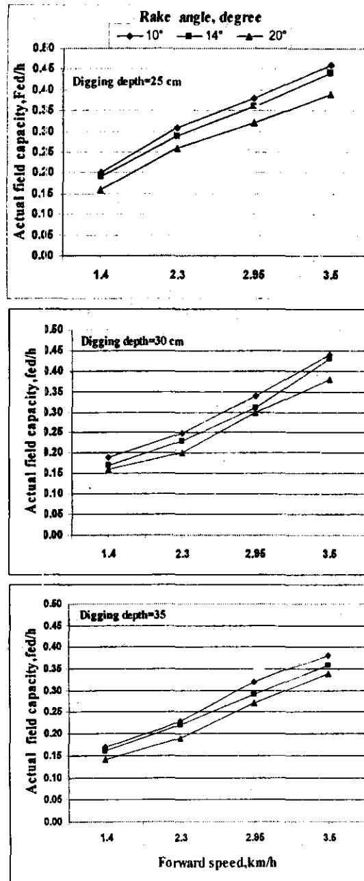
Fig.(3) :Effect of forward speed and rake angle on actual field capacity at different digging depths.
