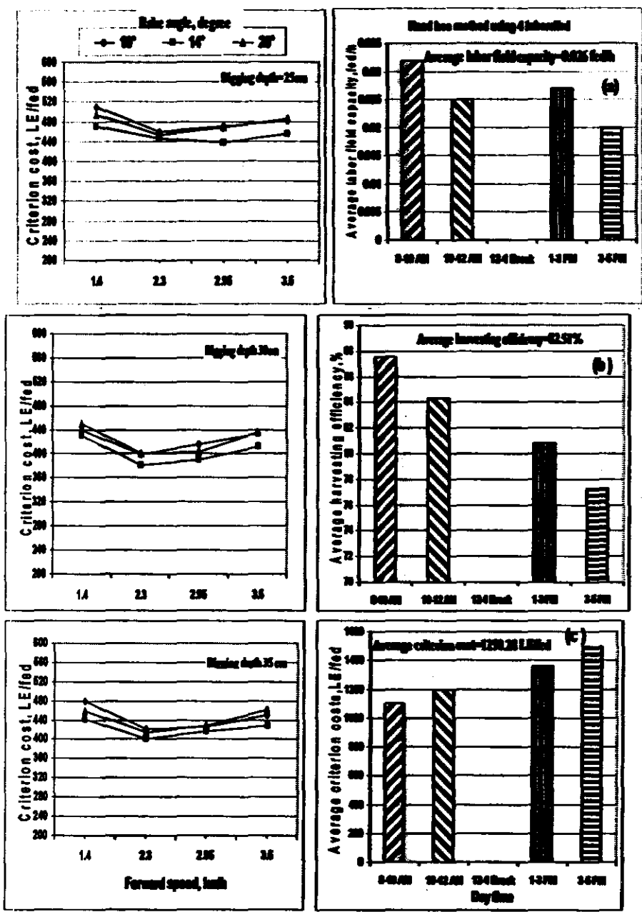
Fig.(6):The criterion cost for mechanical harvesting.
