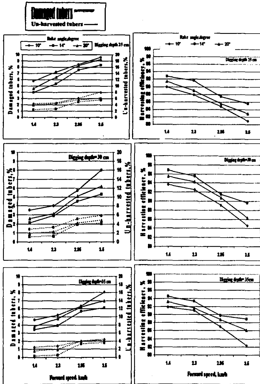
Fig.(4): Effect of forward speed and rake angle on tubers losses and the harvesting efficiency at different digging depths.
