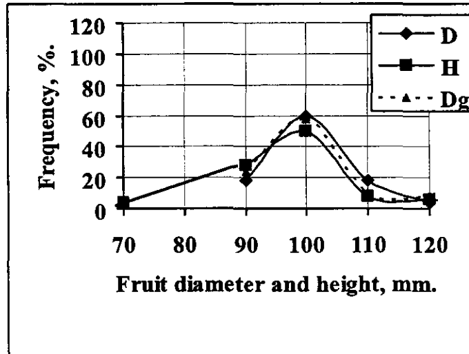
Fig. 3: Frequency curves distribution of fruit dimensions (diameter "D" , geometric diameter "D g "and height "H") of cantaloupe fruits (Charentais variety).
