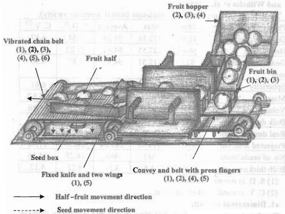
Fig. 2: Diagram demonstrating idea of extracting machine, with the numbers in brackets indicating parameters necessary for design of different parts.
