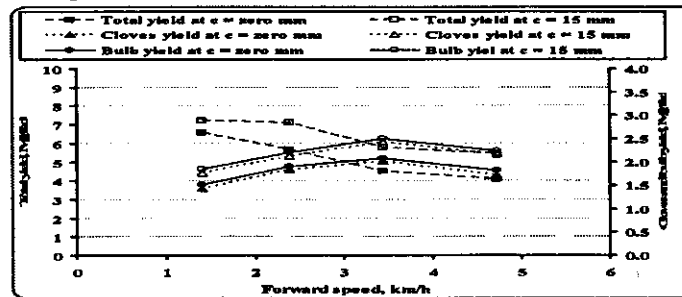
Fig. 10. Effect of forward speed and cutoff clearance on total yield, cloves yield and bulbs yield.
