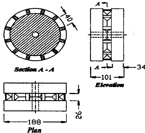
Fig. (3): Metering device of garlic-cloves.
