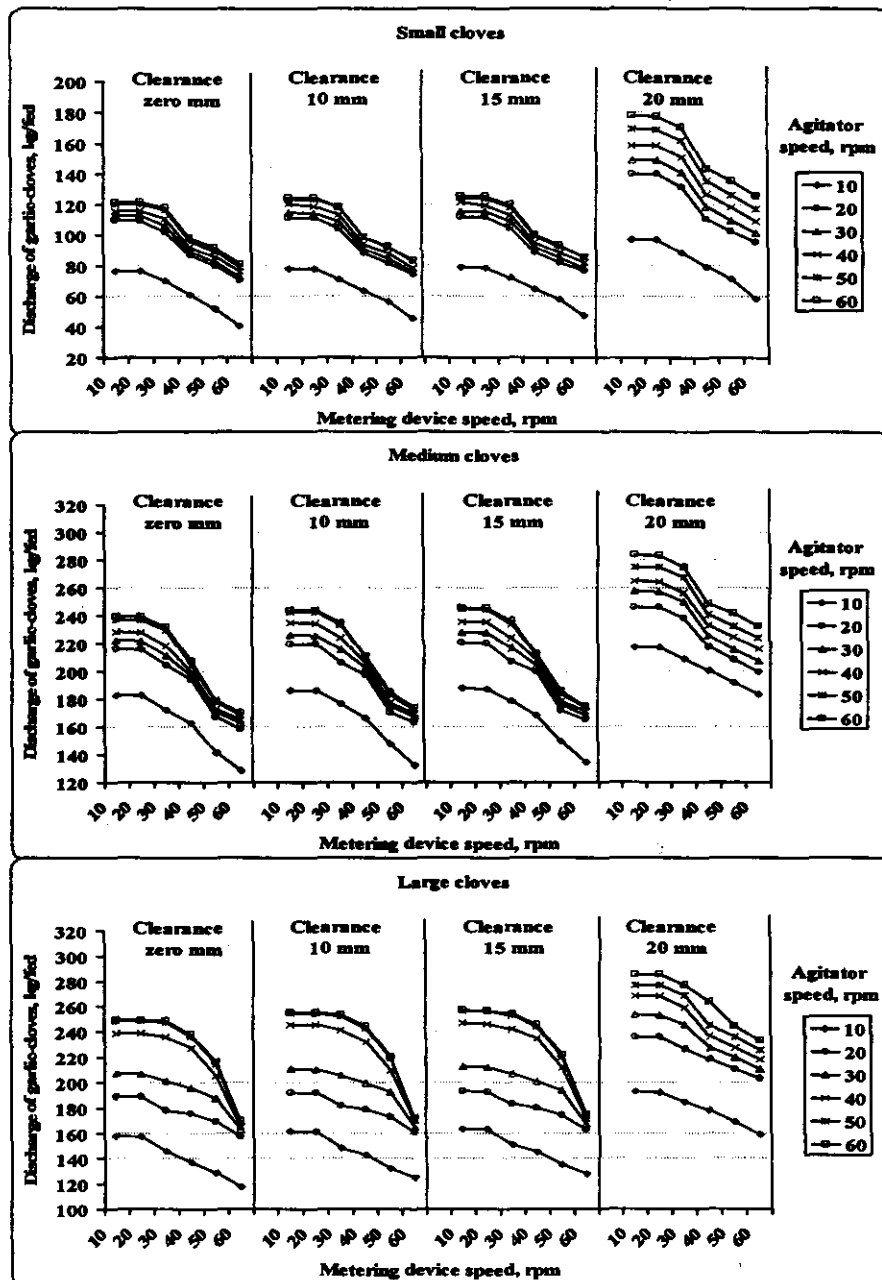
Fig. 4. Effect of metering-device speed, agitator speed and cutoff clearance on discharge of garlic-cloves.
