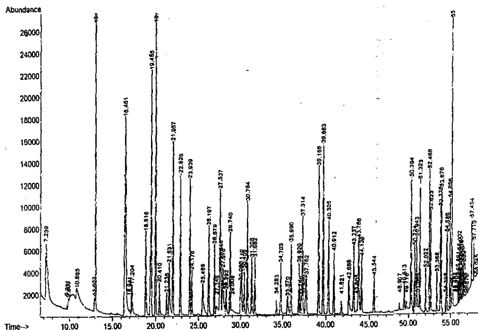
Fig. (1): GC-MS Chromatogram for stander solution of (86) pesticides from (0.1-0.5 µg/ml).
