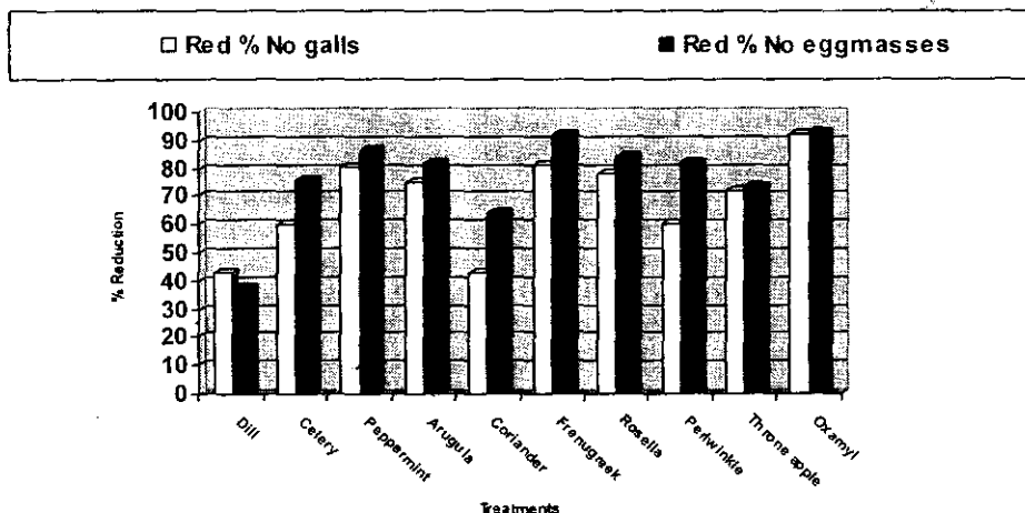
Fig.(2): Reduction percentage of number of root galls and eggmasses, of Meloidogyne incognita infecting eggplant cv. Black Long as affected by nine medicinal and aromatic plant products in comparison with oxamyl under greenhouse conditions.
