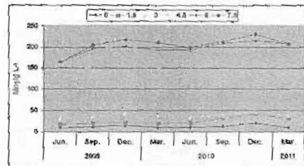
Fig. 5: Mn \mu\text{g L}^{-1} values for Meraga drain water
