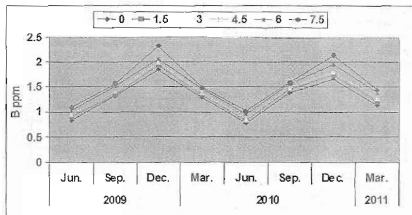
Fig. 3: B ppm values for Meraga drain water.
