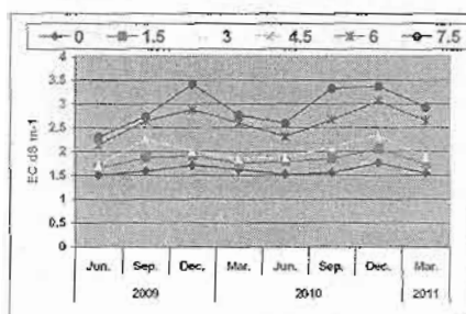
Fig. 1: EC \text{dS m}^{-1} values for Meraga drain water.
