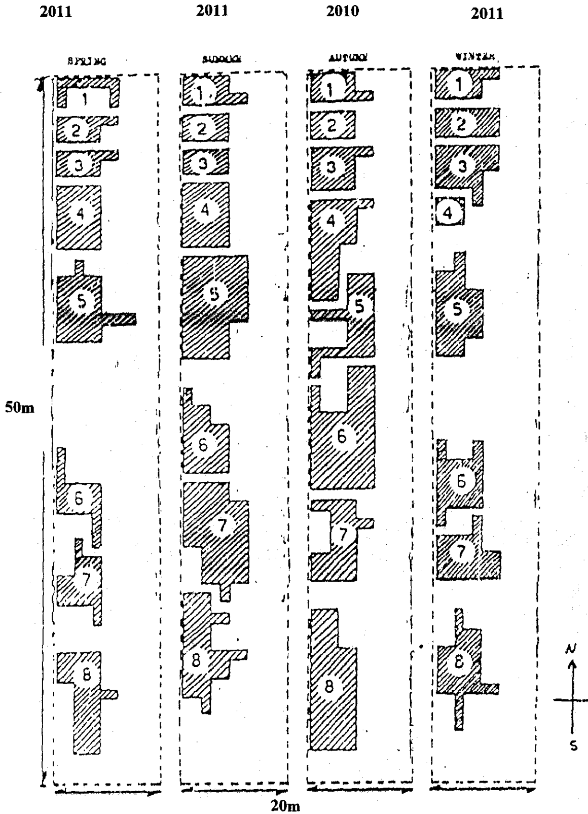
Fig. 2: Delineation of Psammotermes hybostoma foraging territories indicated by weight of consumed traps during October 2010 to November 2011.
