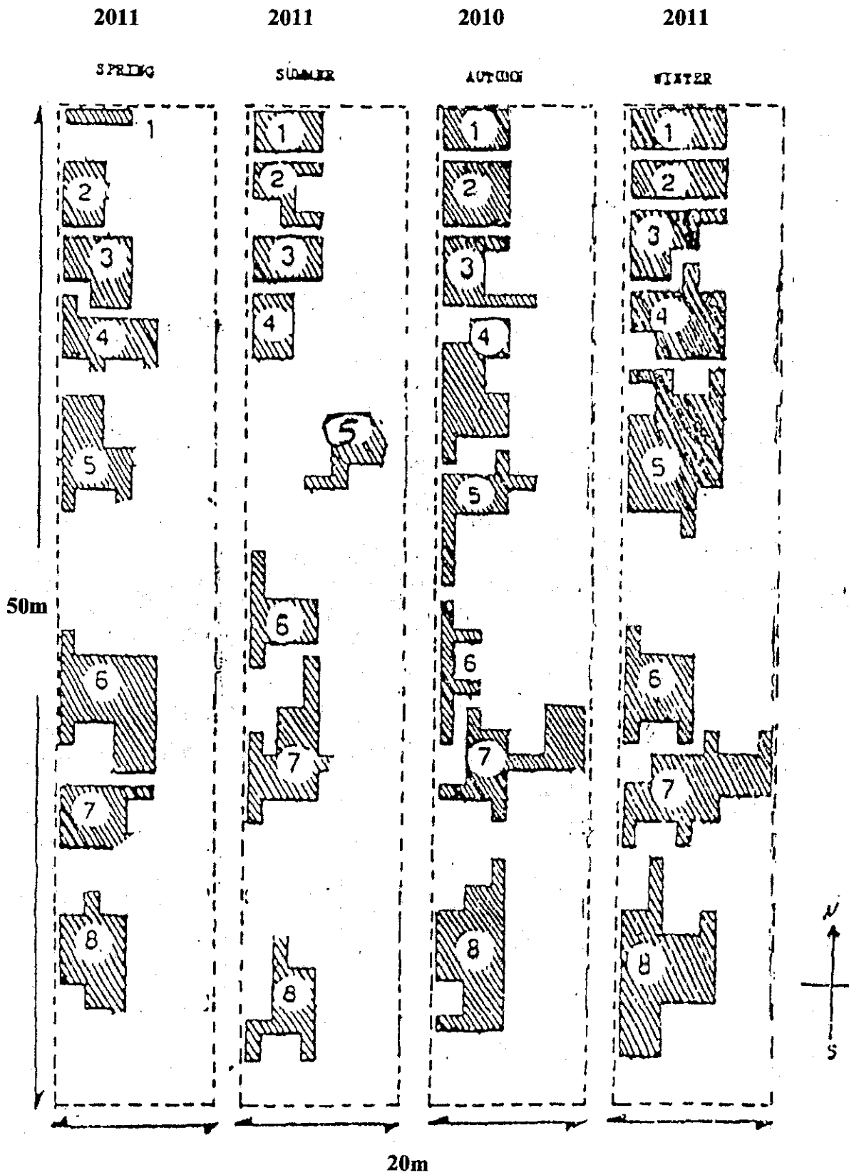
Fig. 1: Delineation of Psammotermes hybostoma foraging territories indicated by number of attracted termitesto the traps during October 2010 to November 2011.
