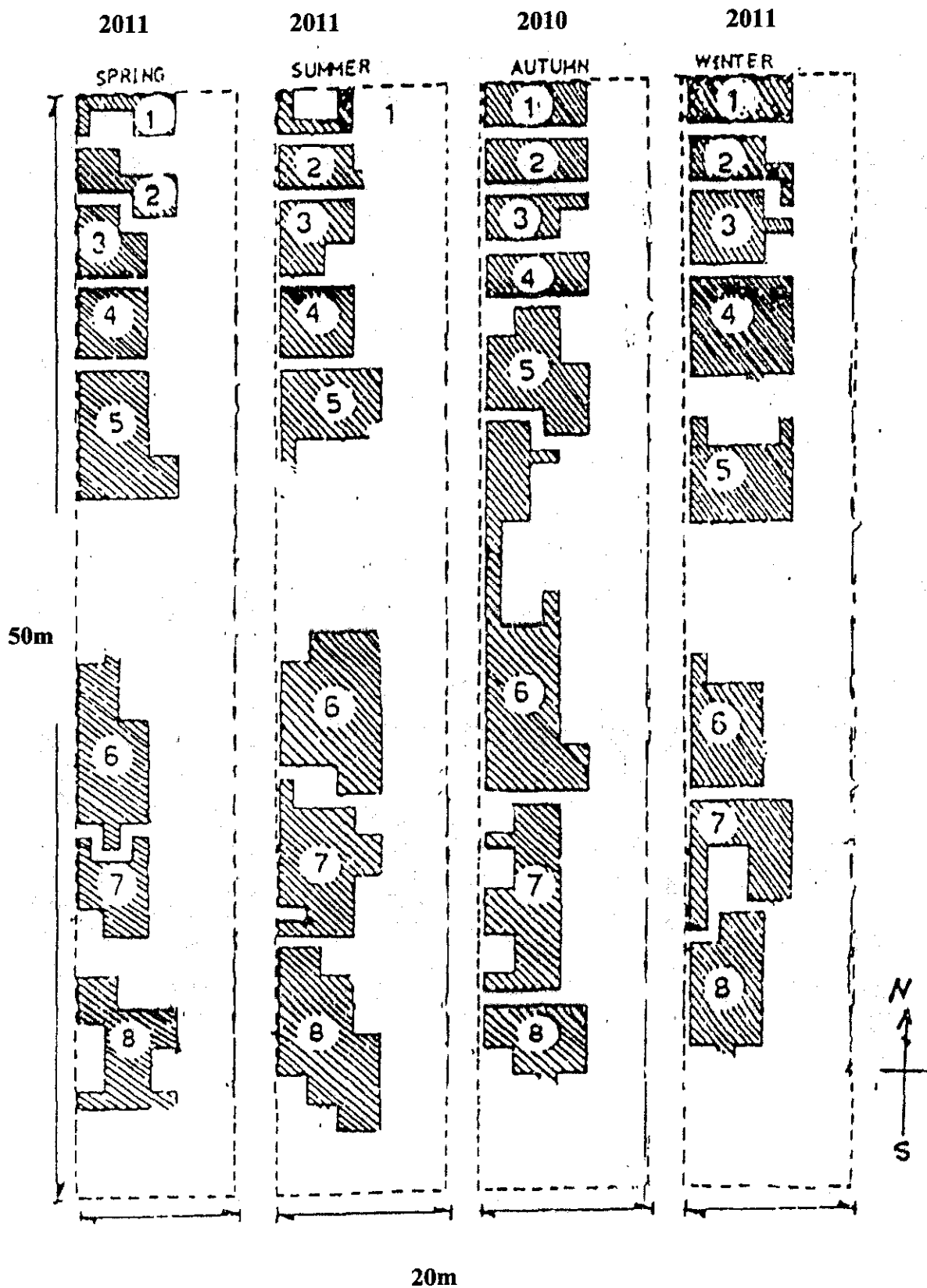
Fig. 3: Delineation of Psammotermes hybostoma foraging territories indicated by weight of translocated soil to the traps during October 2010 to November 2011.
