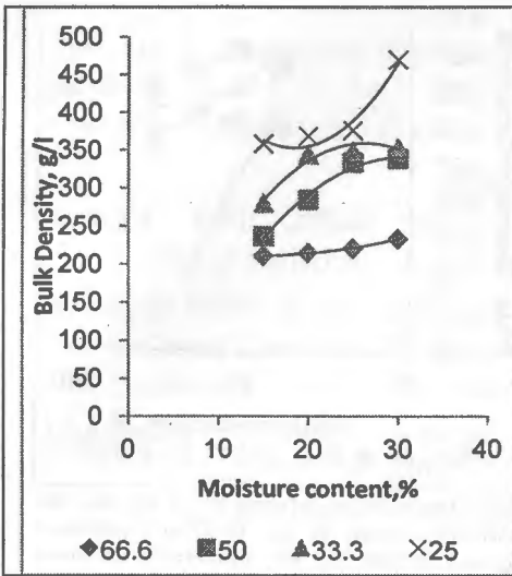
Fig.4. The relation between bulk density and the moisture content of the modified texturized soybean blends for the different treatments before applying the extruder heat insulation.
