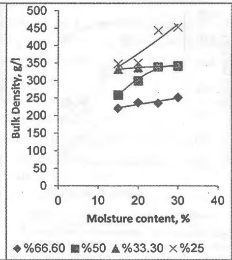
Fig.5. The relation between bulk density and the moisture content of the modified texturized soybean blends for the different treatments after applying the extruder heat insulation
