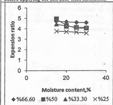
Fig.10. The relation between the Expansion ratio and the moisture content of the modified texturized soybean blends for the different treatments before applying the extruder heat insulation.
