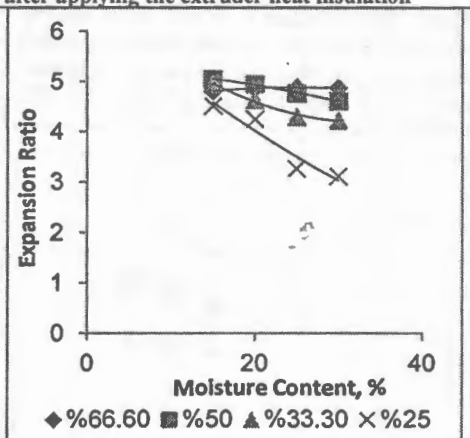
Fig.11. The relation between the Expansion ratio and the moisture content of the modified texturized soybean blends for the different treatments after applying the extruder heat insulation
