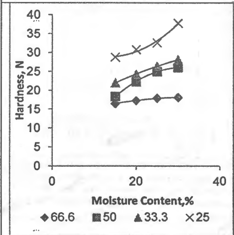
Fig.6. The relation between the hardness and the moisture content of the modified texturized soybean blends for the different treatments before applying the extruder heat insulation
