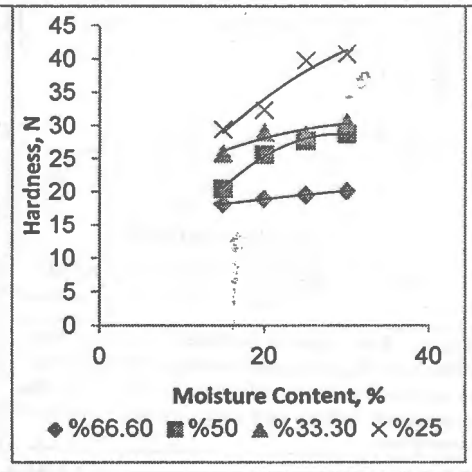
Fig.7. The relation between the hardness and the moisture content of the modified texturized soybean blends for the different treatments after applying the extruder heat insulation
