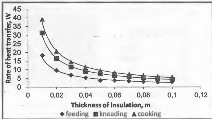
Fig .2. The rate of heat transfer from the insulated barrel to the surrounding air.
