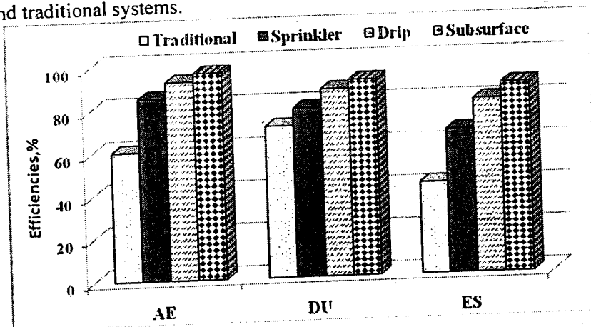
Fig. (1): Application efficiency, distribution uniformity and irrigation system efficiency under different irrigation systems.
