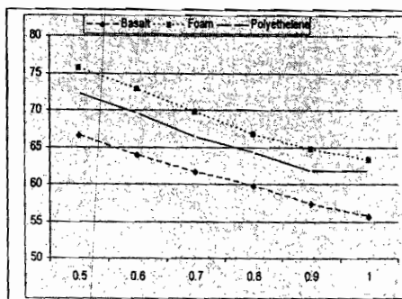
Fig. (1): Effect of Nile water on the filtration efficiency
