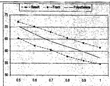
Fig. (2): Effect of west water on the filtration efficiency
