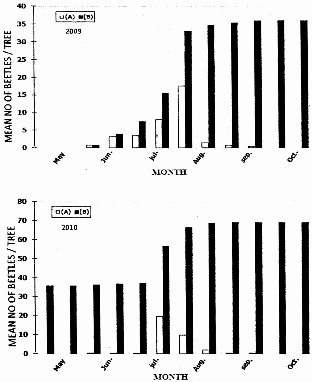
Fig 1:Actual (A) and cumulative (B) mean numbers of M. palmata emerged from casuarina trees in Alexandria region during 2009-2010.
